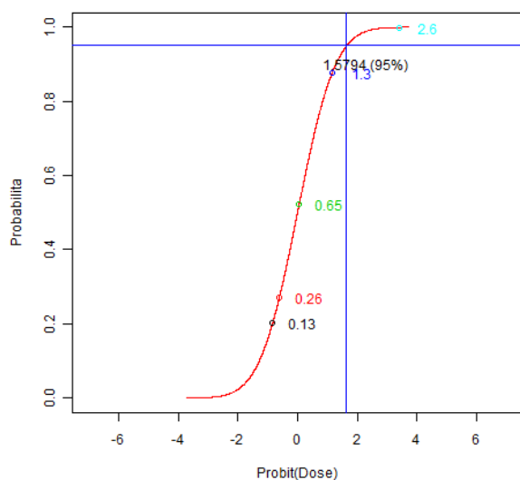
Figure 27. Probit graph
