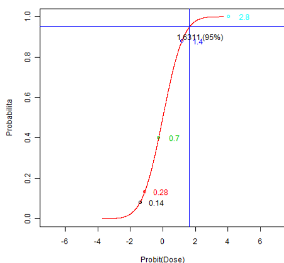
Figure 28. Probit graph
