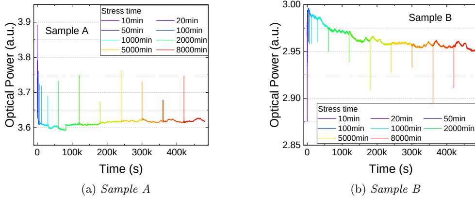
Figure 6.8: Degradation kinetics of electro-luminescence of samples A and B evaluated at the stress current (200mA). The signal is the panchromatic integral of the electro-luminescence of the analyzed devices.
