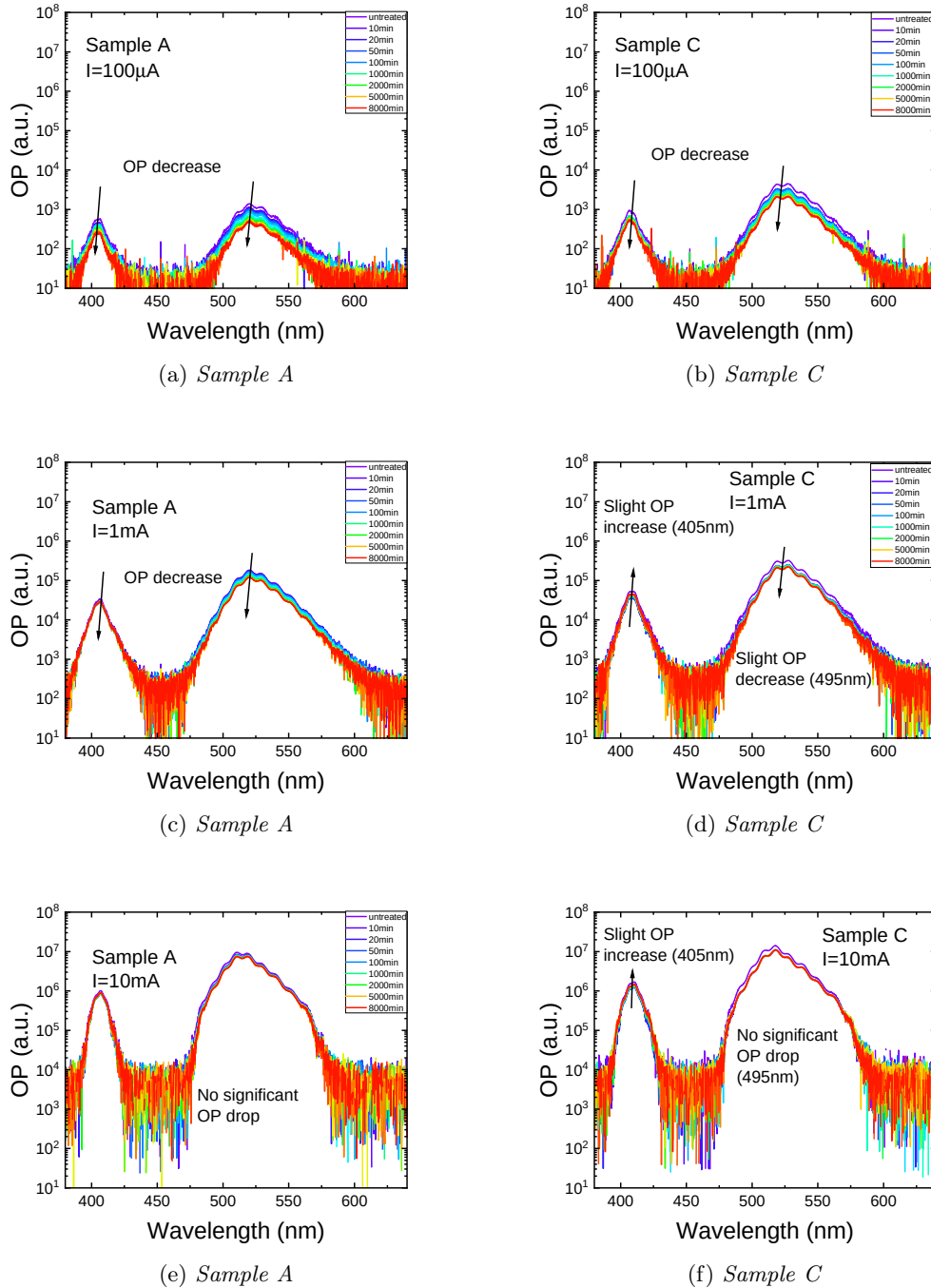
Figure 6.13: Spectra of electro-luminescence measured at different driving current during the constant step-stress at 200mA. All the spectra are taken at room temperature.
