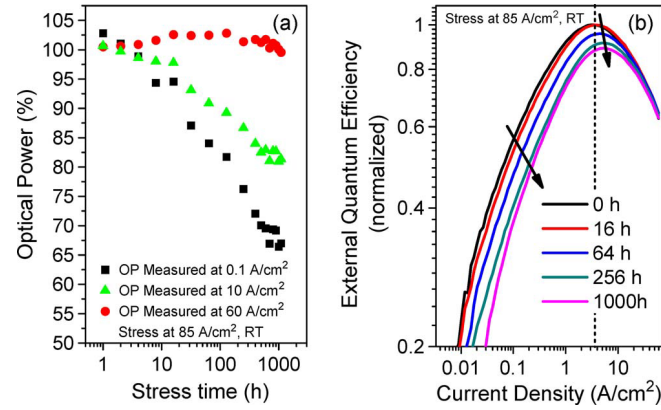
Figure 1.27: (a) Optical power decrease measured (at three different current density levels) during stress of one of the analyzed samples. (b) Efficiency versus injected current characteristics measured during stress of one of the analyzed samples (all the curves were normalized to the peak efficiency measured before stress). Stress conditions are 85 \text{ A/cm}^2 , RT. [11].
