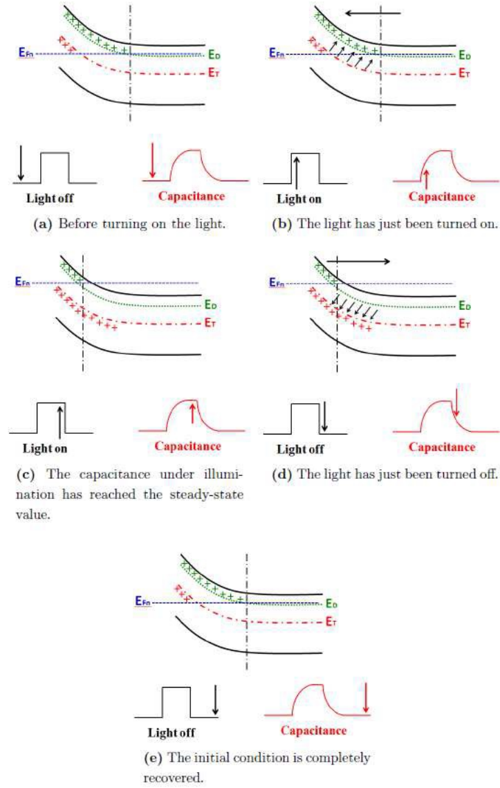
Figure 2.7: Band diagram of a p+n junction during the various steps of a DLOS measurement. A majority carrier trap is supposed to be localized E_T eV below the conduction band. Only the n-side of the junction is shown.
