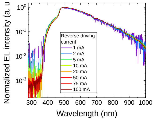
Figure 5.4: Electro-luminescence (EL) in pulsed reverse bias condition at various current levels taken at room temperature (25°C) [64].
