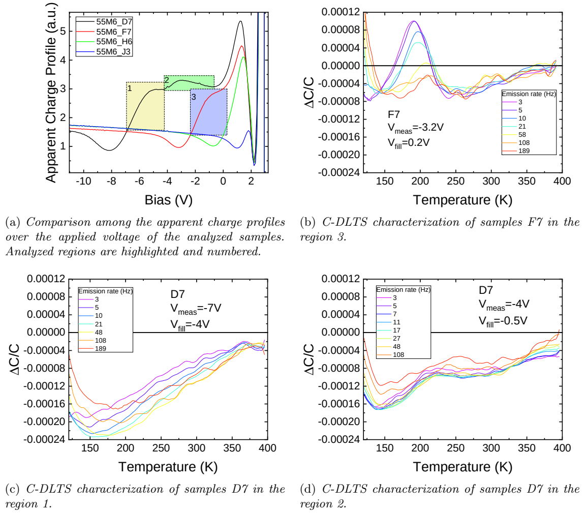
Figure 3.4: C-DLTS results of the different analyzed regions.
