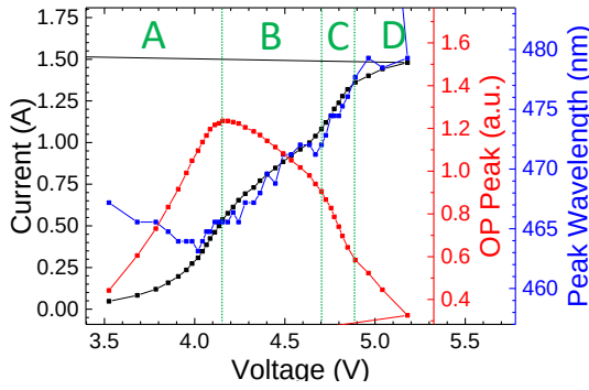
(c) Peak wavelength and peak optical power measured during the pulsed I - V characterization. The correlation between the electrical curve and the wavelength one suggests the strong role of temperature in the device.
