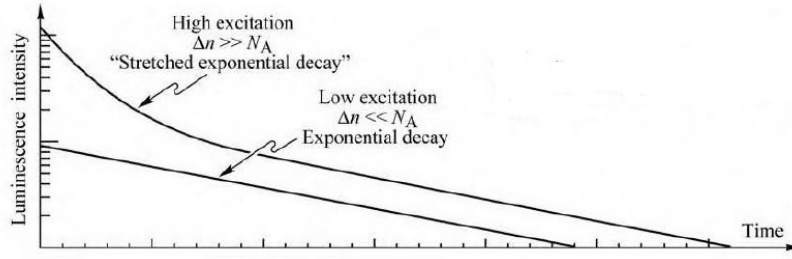
Figure 1.2: Luminescence decay for low and high excitation densities. [28]
