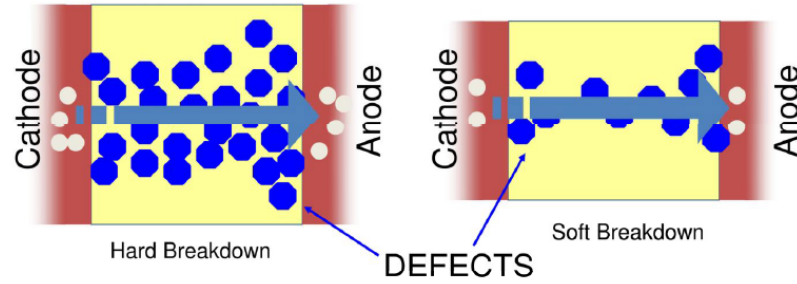
Figure 1.28: Graphical description of the hard and soft breakdown.
