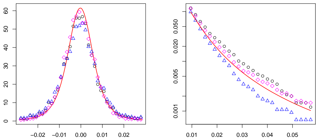
(C) Density of the log-return empirical distribution.
