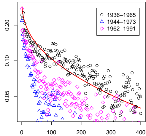
(D) Volatility autocorrelation in subperiods of 30 years.
