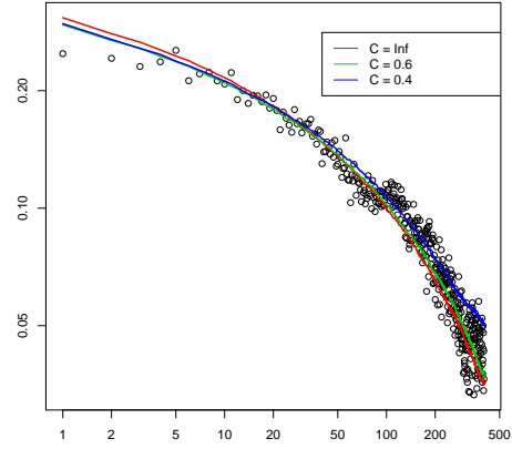
(B) Volatility autocorrelation in the DJIA (1935-2009): log-log plot.
