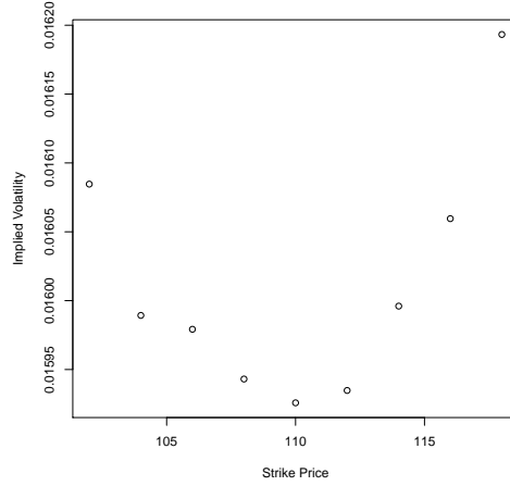
(B) Implied volatility for t_{\bar{j}} - \tau_i(t_{\bar{j}}) = 50 .
