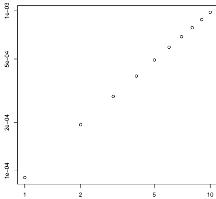
(C) Empirical 2^{\text{nd}} moment \hat{m}_2(h) .
