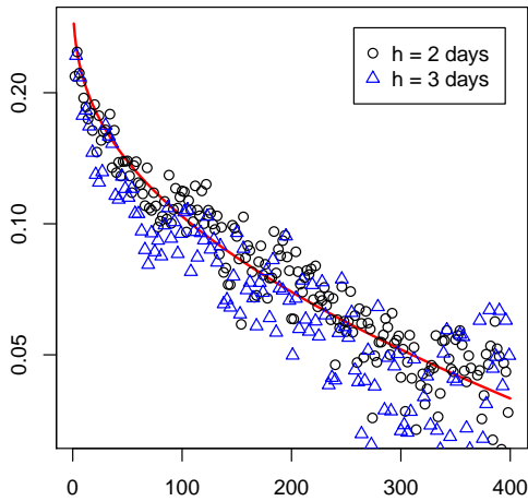
(C) Volatility autocorrelation over h days.
