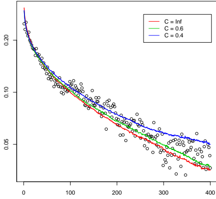
(A) Volatility autocorrelation in the DJIA (1935-2009): log plot.
