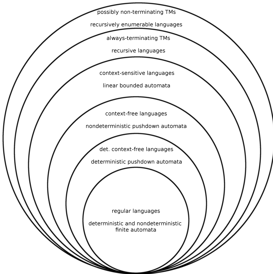
Figure 15.8: An extended Chomsky hierarchy
