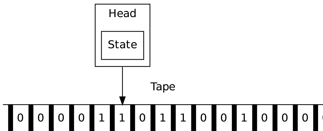
Figure 15.6: Schematic representation of a Turing machine
