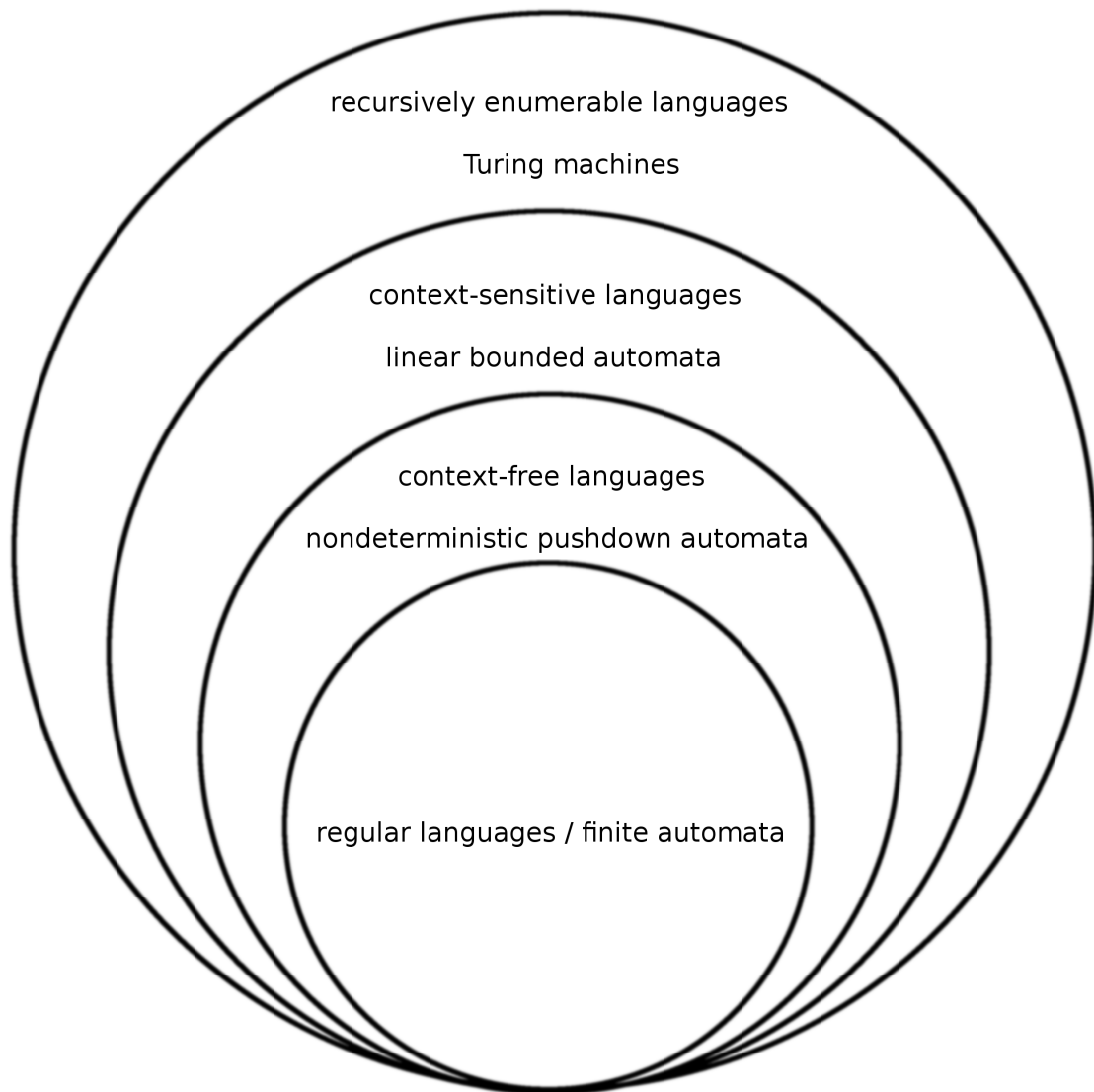
Figure 15.7: The Chomsky hierarchy
