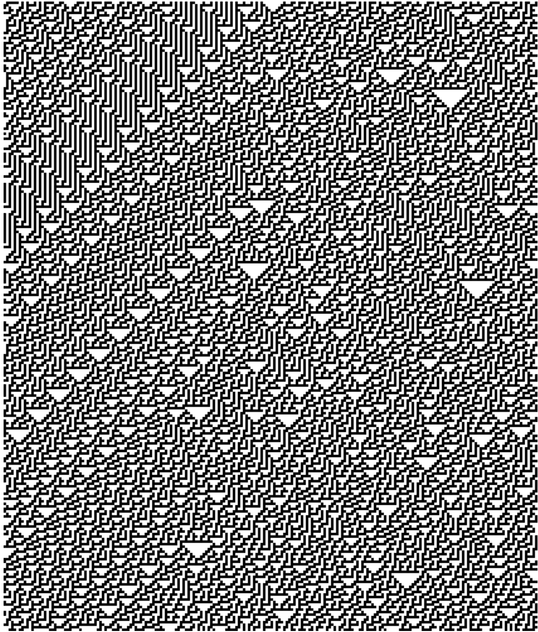
Figure 13.1: chaotic segment of evolution of the elementary CA Rule 30. Time flows from top to bottom, each row of pixels representing the global configuration of the system at each timestep. Each pixel represents the state of one of the elementary parts of the CA, its cells .
