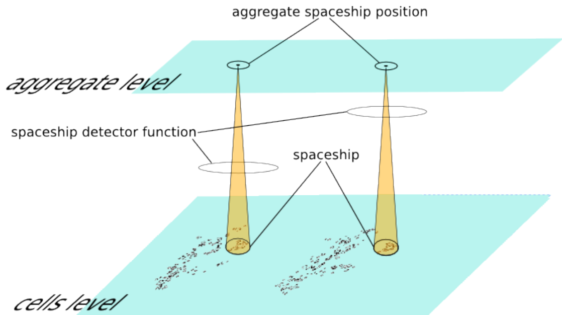
Figure 5.8: The spaceship detector maps any one of the five internal configurations of the period 5 spaceship to a cell of the “aggregate” system, another CA in which each cells represents a spaceship. The position of this cell is the “aggregate” position of the subsystem of the original CA’s dynamical evolution constituting the “spaceship”. The higher level’s dynamics is decoupled from that of the original CA, because the aggregate position of the spaceship advances of 2 pixels every 5 timesteps of the original CA.
