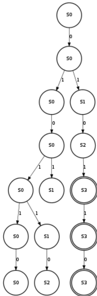
Figure 15.3: Representation of the computational process of a NFA receiving the input string 010110
