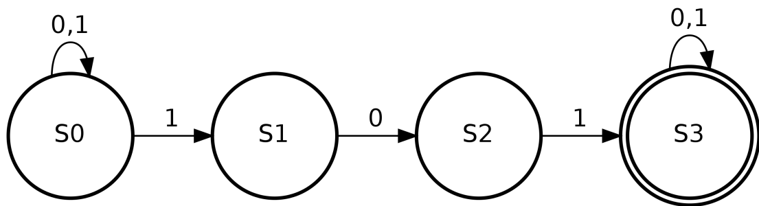
Figure 15.2: State-diagram of a nondeterministic finite automaton
