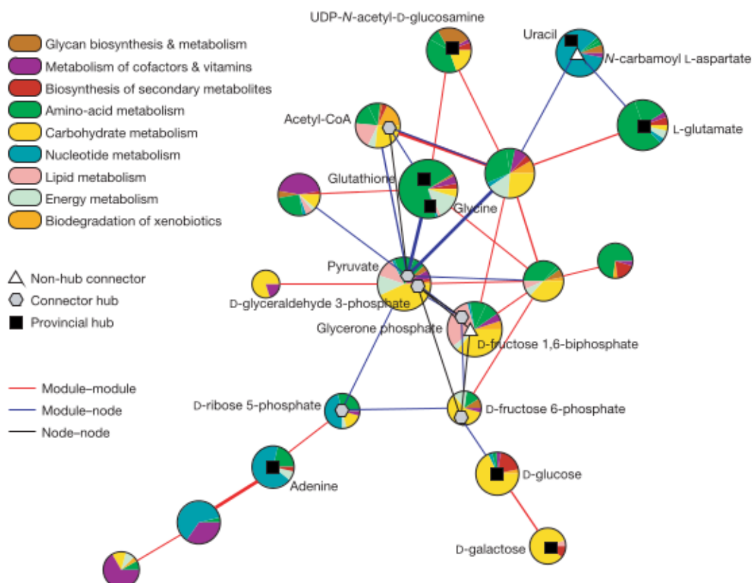
Figure 1.6: high-level modular representation of a metabolic network. (Image taken from Guimerà & Amaral 2005c).
