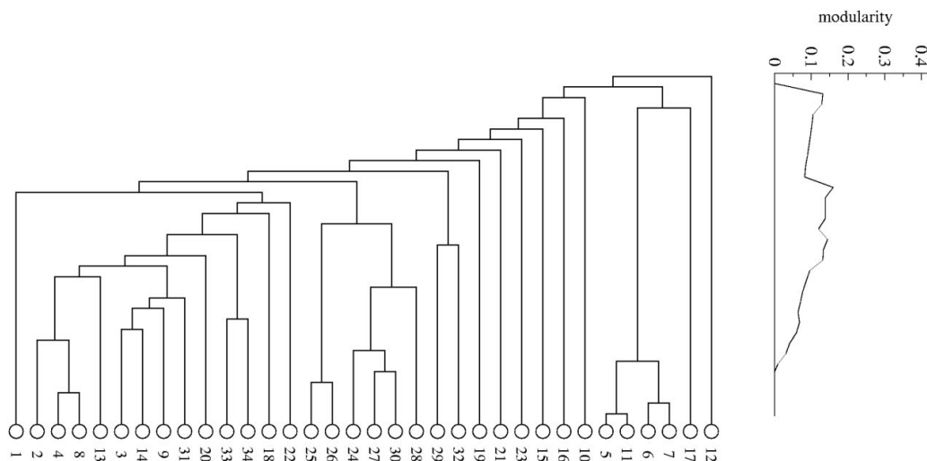
Figure 3.7: . The hierarchical tree of a social network obtained by Newman and Girvan’s with a purposely chosen non optimal algorithm. The graph on the right shows the modularity measure Q . Image adapted from Newman & Girvan (2004).
