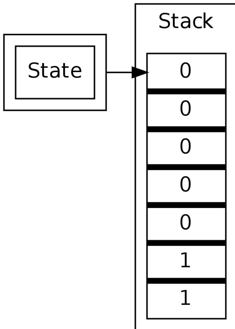
Figure 15.5: Schematic representation of a pushdown automaton
