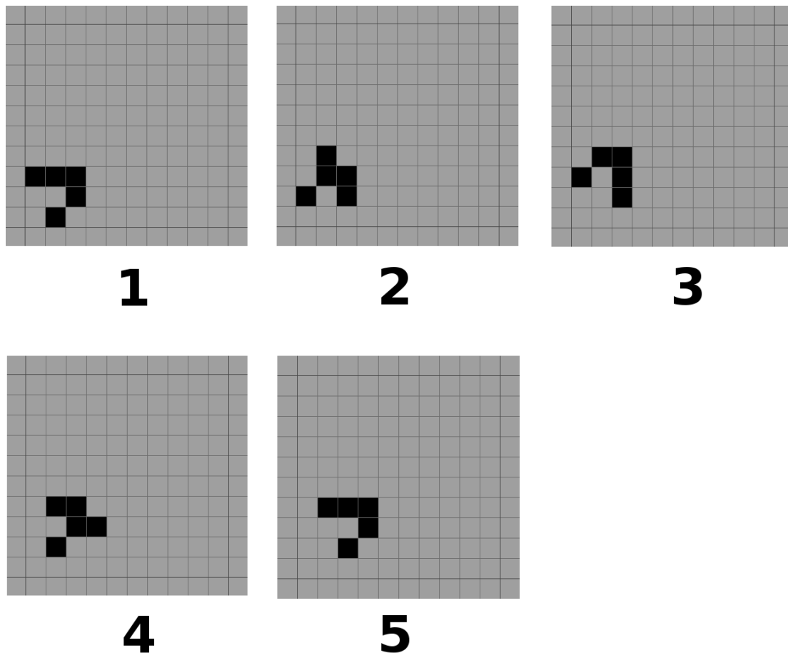
Figure 5.5: a part of the temporal evolution of the Conway’s Game Of Life 2-D CA depicting the basic cycle of a glider , a modular dynamical structure which, if undisturbed, travels across the CA’s array. Time flows from left to right. The glider cycles through four possible configurations (1 to 4) before returning to the initial configuration (step 5). During this cycle the glider travels diagonally 1 cell.
