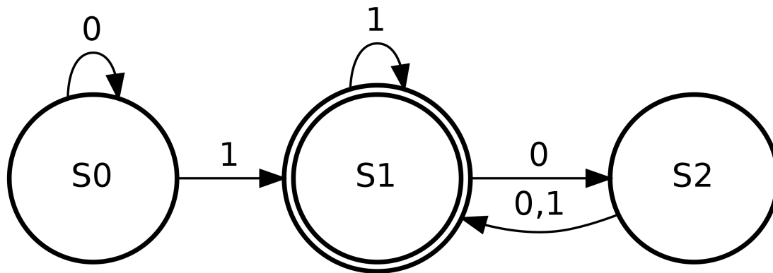
Figure 15.1: State-diagram of a finite automaton
