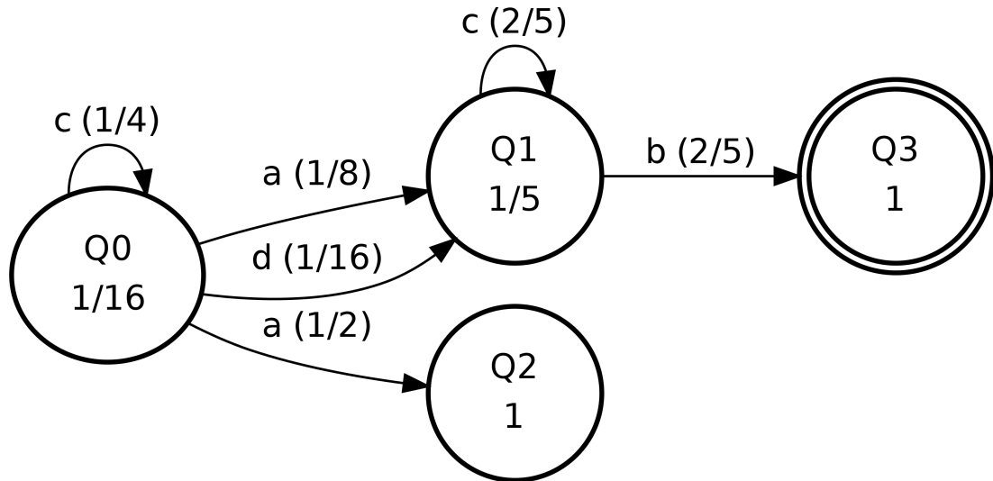
Figure 15.4: State-diagram of a probabilistic finite automaton
