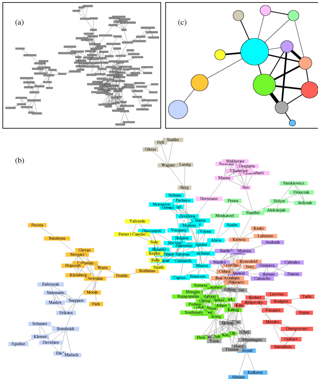
Figure 3.15: (a) The original network of coauthorship between physicists. (b) Detected communities in the original network, identified by colors. (c) The coarse-grained representation of the network: colors indicate which community of the original network each node in the coarse-grained network represents. Image taken from Newman & Girvan (2004).
