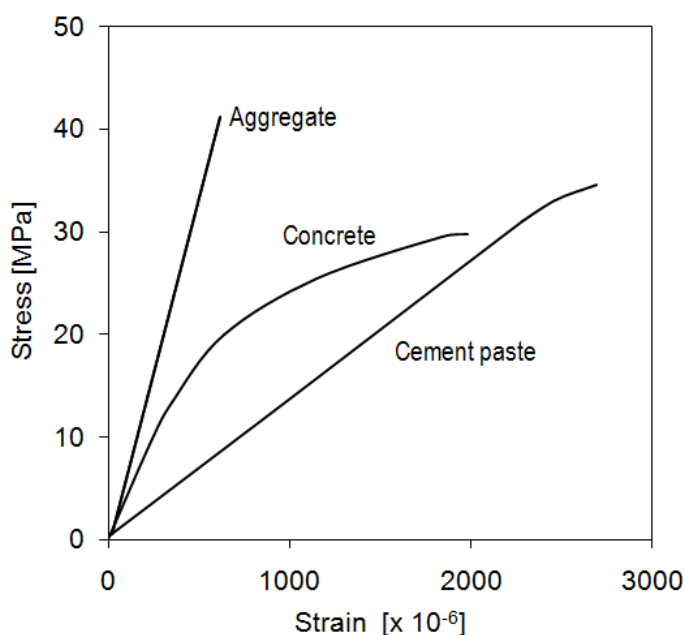
Figure 2.12 – Stress-strain relation for cement paste, aggregate and concrete (Neville, 1996)
