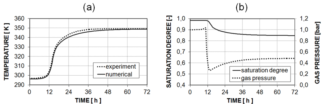
Figure 3.4 - Results of the hydration adiabatic test. Adiabatic temperature (a). Numerical results for the gas pressure and the saturation degree (b)
