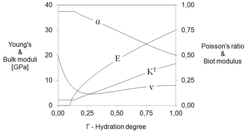
Figure 1.7 - Evolution of the main mechanical properties with hydration
