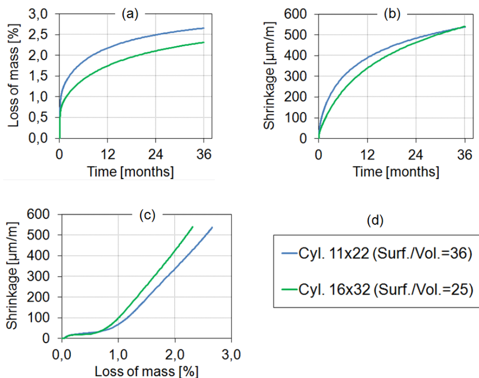
Figure 2.52 - Predicted results during 36 months for the reference cylinder (11Ø×22) and the bigger one (16Ø×32): loss of mass (a), drying shrinkage (b), loss of mass versus drying shrinkage curves (c), legend of the graphs (d).
