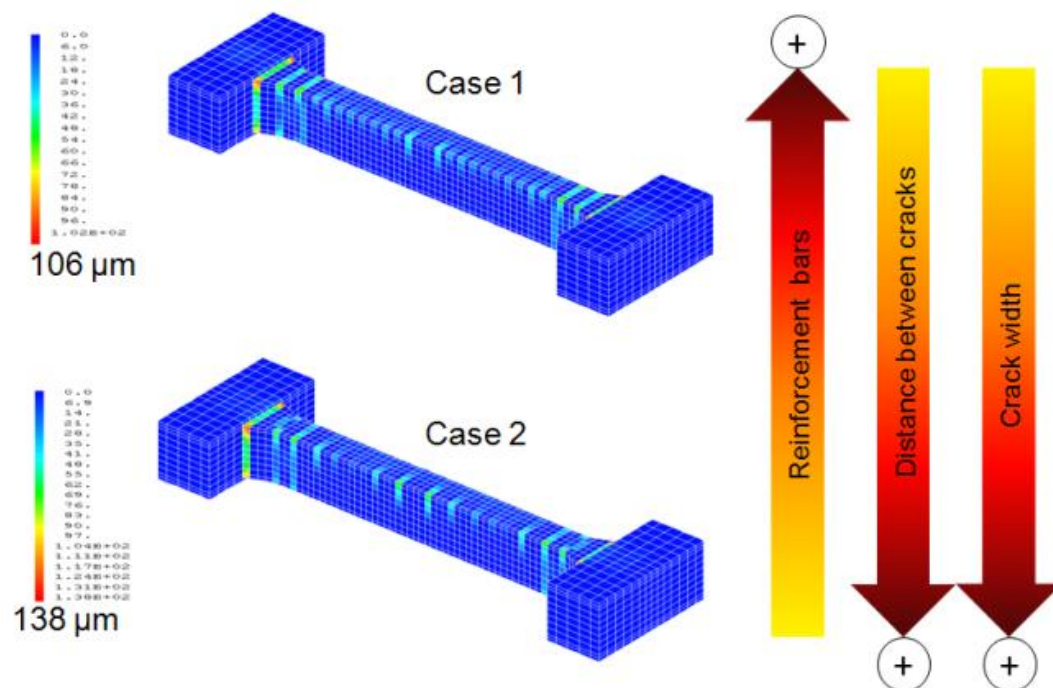
Figure 3.13 - Estimation of cracks width two months after the cast for two specimens with different amount of longitudinal bars reinforcement. Specimen 1 more reinforced than specimen 2.
