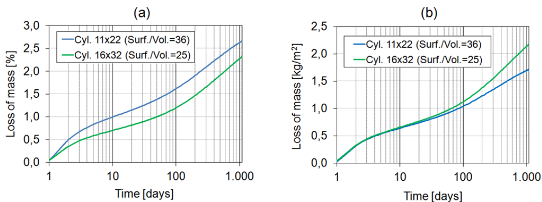
Figure 2.53 - Predicted results during 1080 days for the reference cylinder (11Ø×22) and the bigger one (16Ø×32): loss of mass [% of the initial weight] (a), loss of mass [kg/m 2 ] (b).
