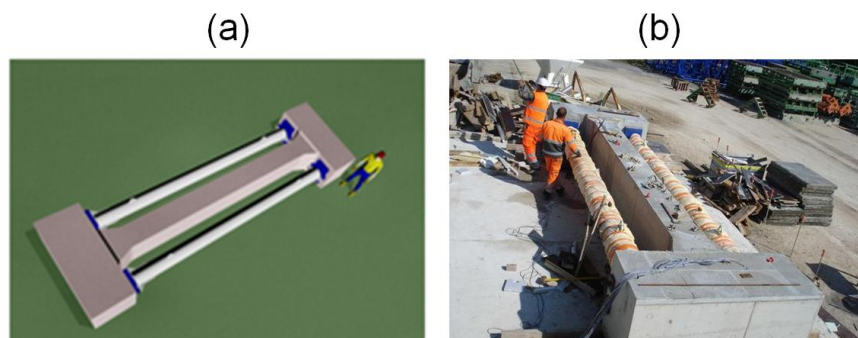
Figure 3.1 - 3D specimen model (a). Photo of the specimen after the removal of formwork and thermal isolation (b). Images from ConCrack home page
