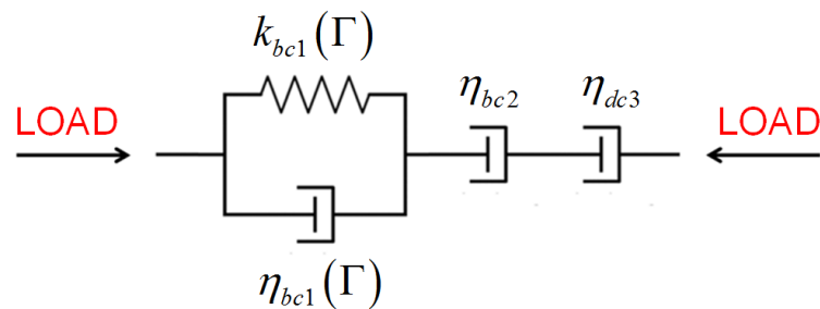
Figure 2.61 - Creep rheological model
