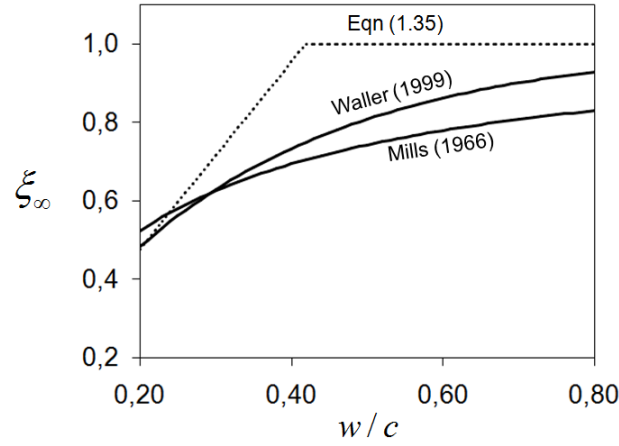
Figure 1.4 – Maximum hydration degree over the w/c ratio. Value given by eqn (1.35) and estimations obtained using eqs (1.36).
