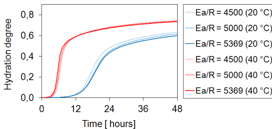
Figure 2.11 – Hydration degree during 48 hours for the three considered values of the activation energy. Two curing temperatures are considered: 20 ^{\circ}\text{C} (blue lines) and 40 ^{\circ}\text{C} (red lines).
