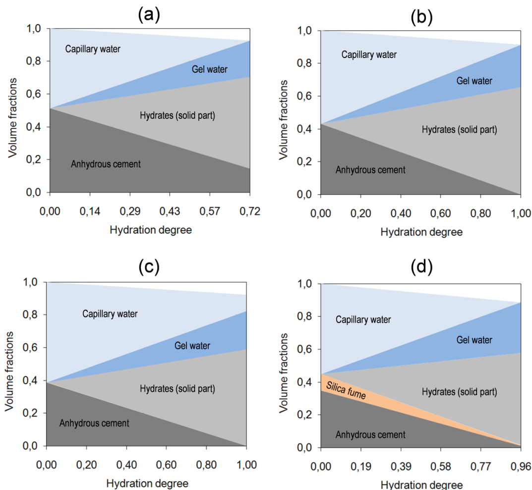
Figure 2.5 – Volume fractions over hydration of unhydrated cement, silica fume, capillary water, gel water and hydrates (solid part) for four cement pastes: w/c=0.30 (a); w/c = 0.42 (b); w/c = 0.5 (c); w/c = 0.5 and s/c = 0.2 (d).
