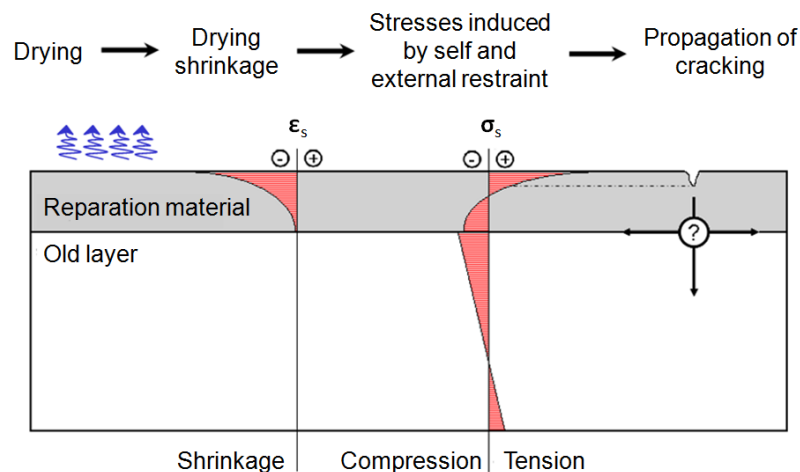
Figure 3.15 - Drying cracking due to self and external restraint in a repair (adapted from Molez, 2003)
