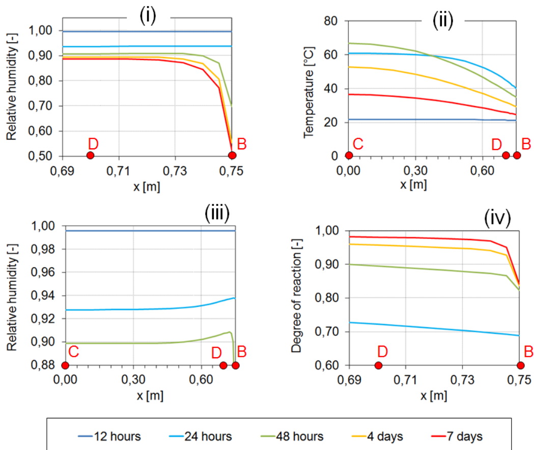
Figure 2.41 – Numerical results over the line L CB at different times (12 hours, 24 hours, 48 hours, 4 days and 7 days). Relative humidity near the edge (i); temperature over the full L CB (ii); relative humidity over the full L CB (iii); degree of reaction near the edge (iv).
