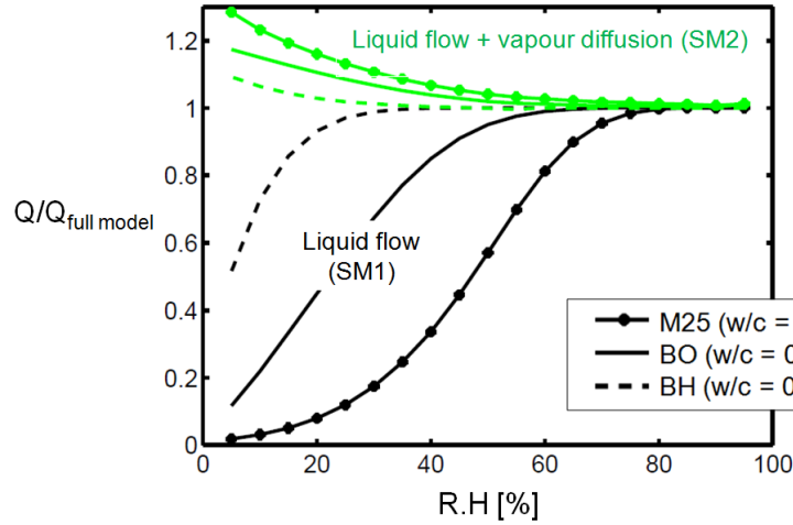
Figure 2.34 – Ratio between the loss of mass after 1000 days of drying calculated using the two simplified models (SM1 and SM2) and that calculated using the full model (FM). Three concretes have been considered (M25, BO and BH). The initial relative humidity has been set equal to h_0 = 99\% and the resulting ratios are plotted as functions of the imposed external relative humidity h_{ext} . Image readapted from Thiery et al. (2007).
