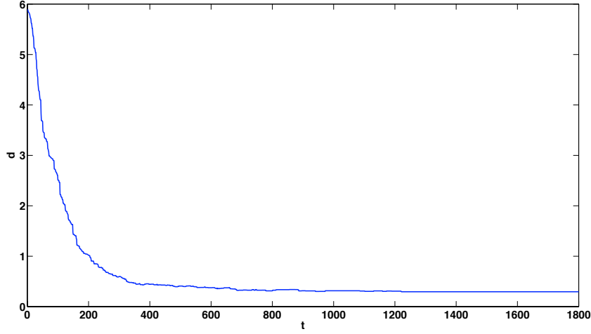
Figure 6.1: Behavior of d for a connected random graph with N = 50 in case of deterministic quantizers and of partially quantized strategy.
