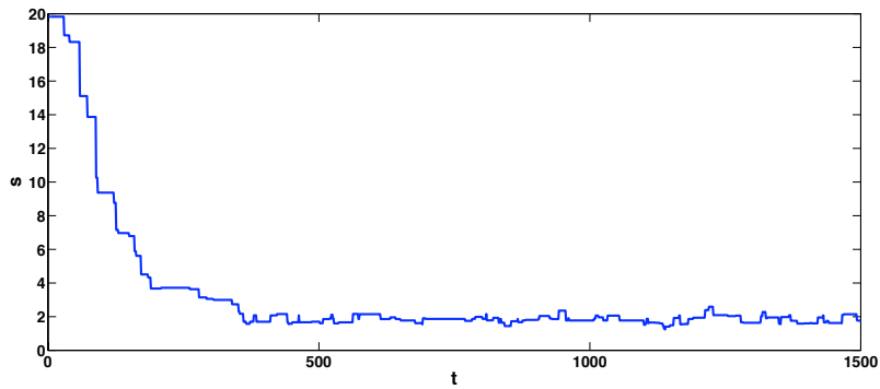
Figure 6.6: Behavior of s for a connected random geometric graph with N = 50 .
