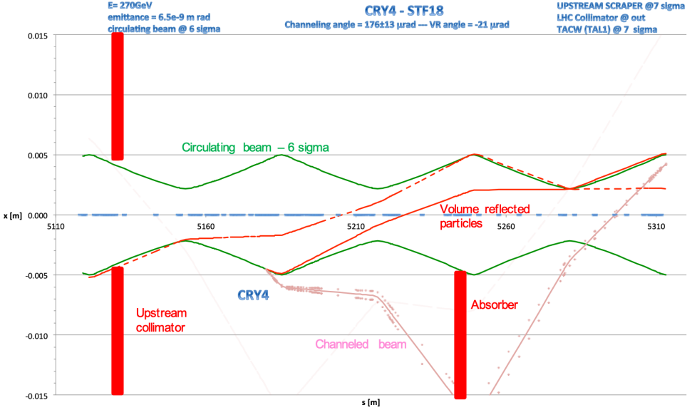
Fig. 33. (Color online) Tracking of the beam in the SPS. In green the circulating beam at 6\sigma with energy 270 GeV and emittance 6.5 \times 10^{-9} m · rad. In brown the beam channeled by the crystal with 176 \mu\text{rad} . In red the volume-reflected beam at the first turn. In light orange the volume-reflected beam at the second turn.
