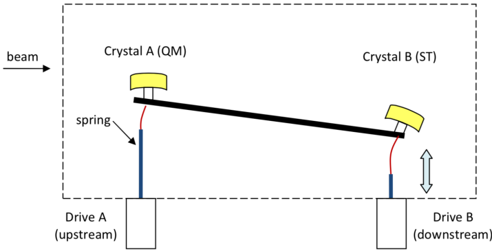
Fig. 7. The IHEP-goniometer kinematics. The scheme shows the Crystal A (upstream) alignment: the position is controlled by an equal, synchronous motion of the Drive A and B; the angle by the Drive B, only.
