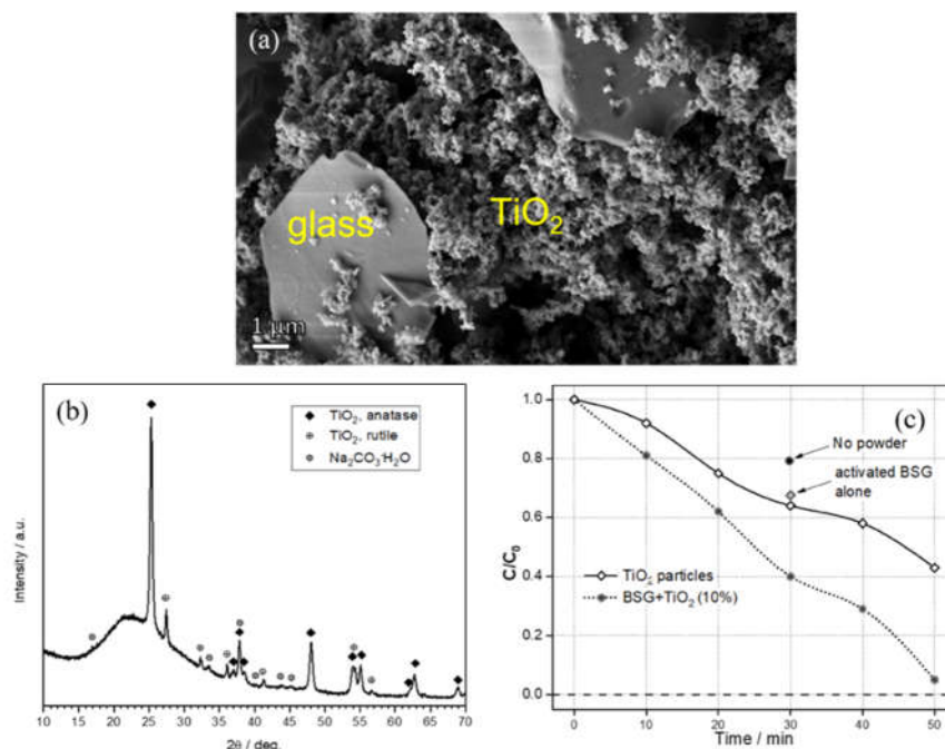
Figure 7. (a) Detail of glass/ \text{TiO}_2 composite granule; (b) diffraction analysis of hardened glass/ \text{TiO}_2 suspension; (c) evolution of relative concentration with increasing UV exposition time operating with \text{TiO}_2 photocatalyst.
