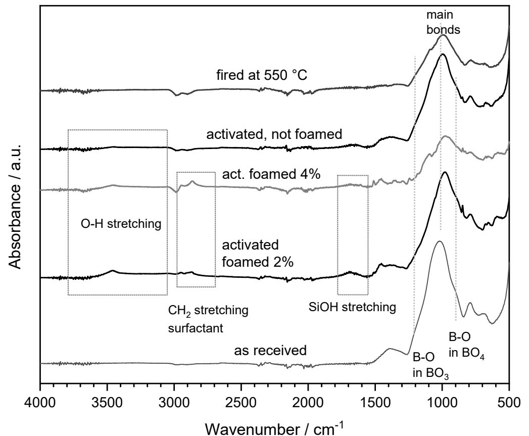
Figure 3. Fourier transform infrared (FTIR) analysis of boro–alumino–silicate glass in the as-received state, after activation and after firing.
