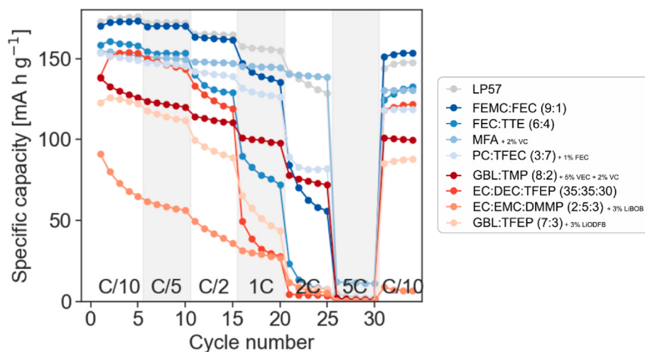
Fig. 3. Rate capability of the electrolytes based on organophosphorus compounds (red traces) and fluorinated carbonates, esters and ethers (blue traces). (For interpretation of the references to colour in this figure legend, the reader is referred to the Web version of this article.)
