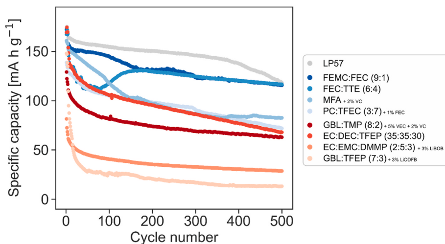
Fig. 2. Galvanostatic cycling performance of the non-flammable electrolytes studied in this work, grouped into phosphate/phosphonate-based and fluorinated carbonate/ester/ether-based, with LP57 shown as a benchmark.
