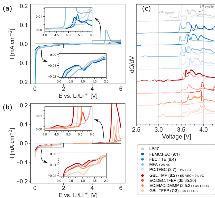
Fig. 1. Linear sweep voltammetry (LSV) of the (a) hydrofluorocarbon-based and (b) phosphate/phosphonate-based non-flammable electrolytes studied in this work. Anodic and cathodic sweeps were done using carbon-coated copper and carbon-coated aluminum working electrodes, respectively. (c) dQ/dV plots of the 1st and 5th cycles (at C/10) of NMC622|graphite containing each electrolyte.
