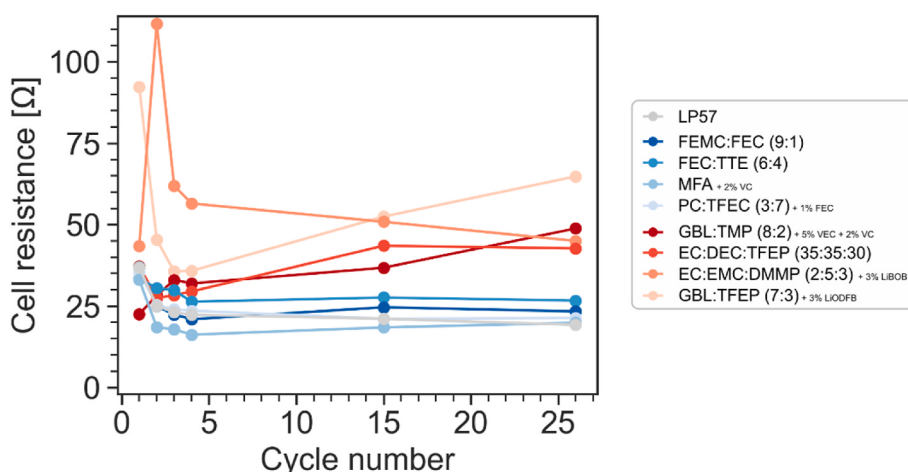
Fig. 4. Internal resistance of NMC622/graphite cells containing various non-flammable electrolytes during cycling, as obtained by intermittent current interruption. Resistance values represent means during charge steps. Cycles 1–2, 15 and 26 (containing ICI steps) were carried out at a C-rate of C/10, while cycles 3–4 were carried out at C/5. Cycles 5–14 and 16–25 (without ICI) were carried out at a C-rate of C/2.
