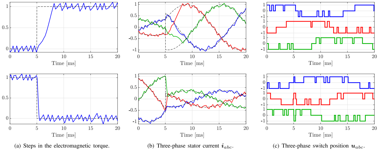
Fig. 13. HIL results during torque reference step changes with the proposed FCS-MPC for N = \{5, 1\} . A simultaneous -50% variation in both X_{ls} and X_{lr} is introduced while the estimation algorithm is active. The average switching frequency is f_{sw} \approx 250 Hz.
