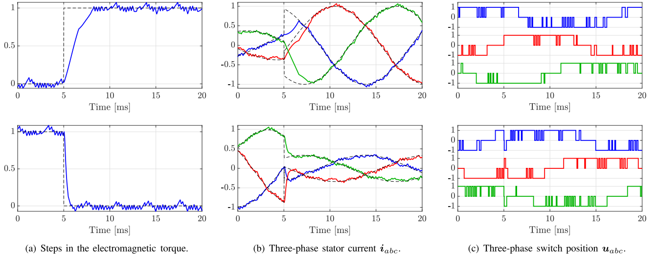
Fig. 14. HIL results during torque reference step changes with the proposed FCS-MPC for N = \{5, 1\} . A simultaneous -50\% variation in both X_{ls} and X_{lr} is introduced while the estimation algorithm is inactive . The average switching frequency is f_{sw} \approx 545 Hz.
