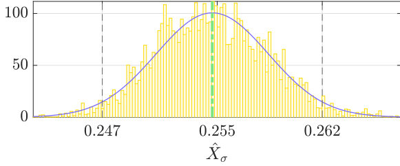
Fig. 10. The normalized histogram and the posterior predictive probability distribution of the \hat{X}_\sigma values recorded over a span of 10 s. The 95 % confidence interval for the next estimation is \text{CI}_{95} = [0.247, 0.262] which is within the range of \pm 3\% from the nominal machine reactance X_\sigma^{\text{mach}} = 0.2548 p.u.
