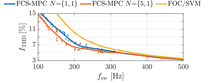
Fig. 5. Trade-off between current THD I_{\text{THD}} and switching frequency f_{sw} for FCS-MPC with horizon combinations N = \{1, 1\} and \{5, 1\} for T_s = 30 \mu\text{s} , and for FOC with SVM.
