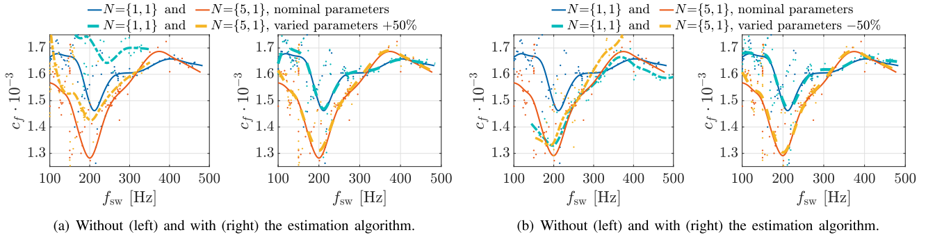
Fig. 12. HIL results for the performance metric c_f as a function of the switching frequency f_{sw} for horizon combinations N = \{1, 1\} and \{5, 1\} . A simultaneous +50% variation in both X_{ls} and X_{lr} is introduced in Fig. 12(a), whereas a simultaneous -50% variation is introduced in Fig. 12(b) for the same reactances. Each individual HIL test—indicated by a dot—corresponds to a real-time simulation of 2 s.
