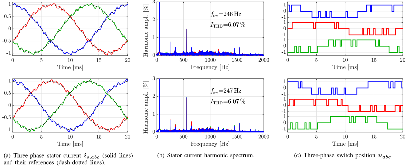
Fig. 11. HIL results at steady-state operation with the proposed FCS-MPC for N = \{5, 1\} . Top row: nominal parameters. Bottom row: a simultaneous -50% variation in both X_{ls} and X_{lr} is introduced while the estimation algorithm is active, resulting in effectively the same performance.
