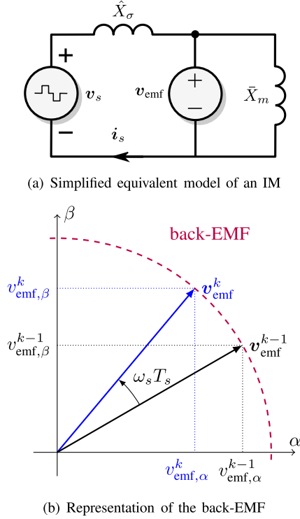
Fig. 7. Principle of the proposed estimation algorithm.
