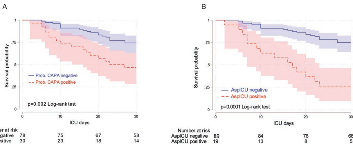
Figure 2. Kaplan-Meier survival curves for 30-day mortality from ICU admission. Patients were stratified as having probable CAPA (A) or PIPA AsplICU criteria fulfilled (B). Abbreviations: CAPA, coronavirus-associated pulmonary aspergillosis; ICU, intensive care unit; PIPA, putative invasive pulmonary aspergillosis; prob., probable.
