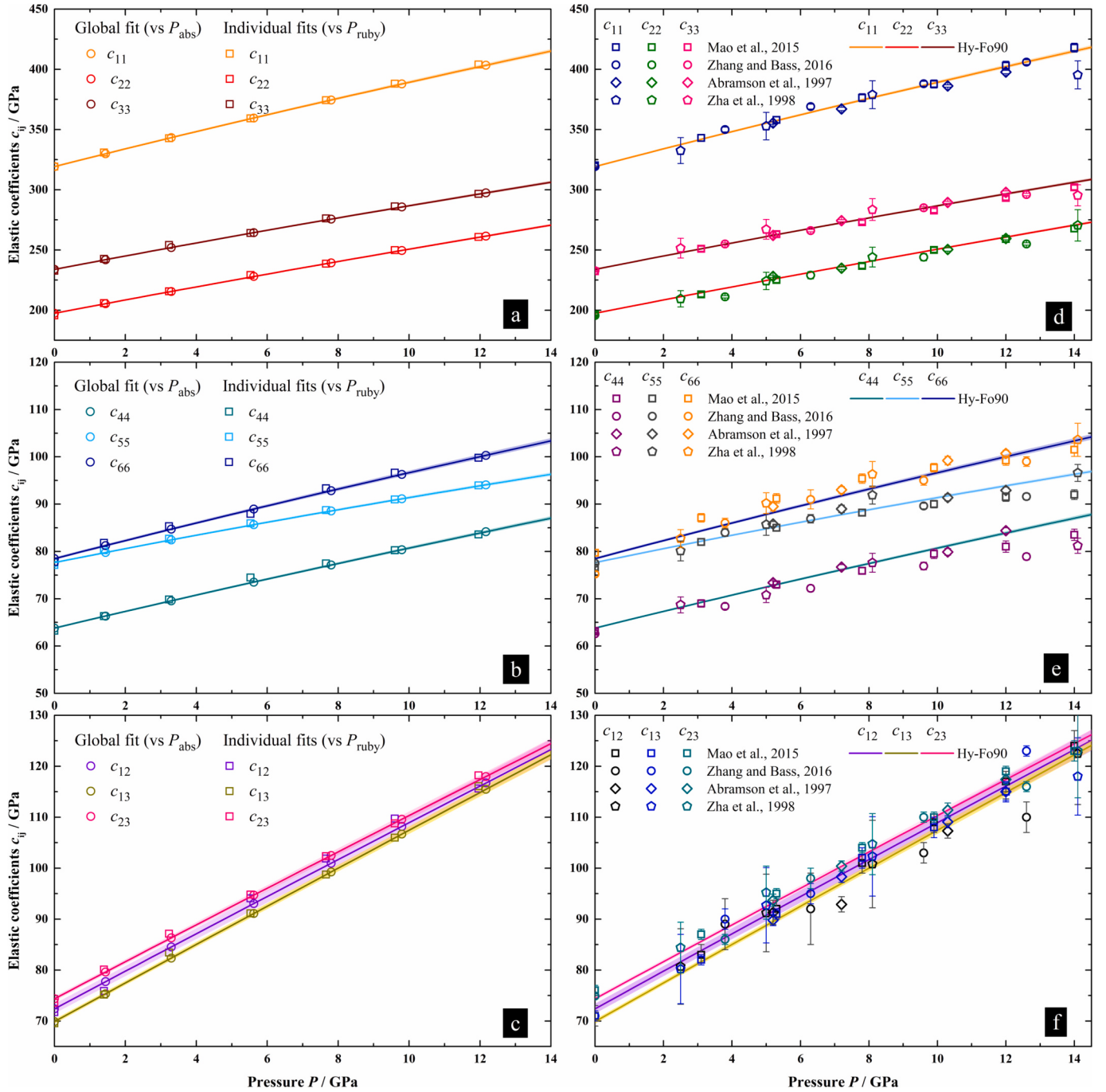
Fig. 4. (a-b-c) Comparison of the c_{ij} values obtained through the global fit (open circles) and individual fits (open squares), showing values typically identical within two standard deviations (Table 2); the solid lines represent third-order EoS fits of each c_{ij} (global fit parameters) (Table 3). (d-e-f) Comparison of the c_{ij} of anhydrous Fo90 olivines selected from previous literature (Abramson et al., 1997; Mao et al., 2015; Zha et al., 1998; Zhang and Bass, 2016; Supplementary Table S2), and the fit curves for each c_{ij} (global fit parameters) of hydrous Fo90 olivine obtained in this study. Note that the fits of the experimentally determined c_{ij} s for hydrous olivine and the c_{ij} s of the corresponding anhydrous phase are nearly identical.
