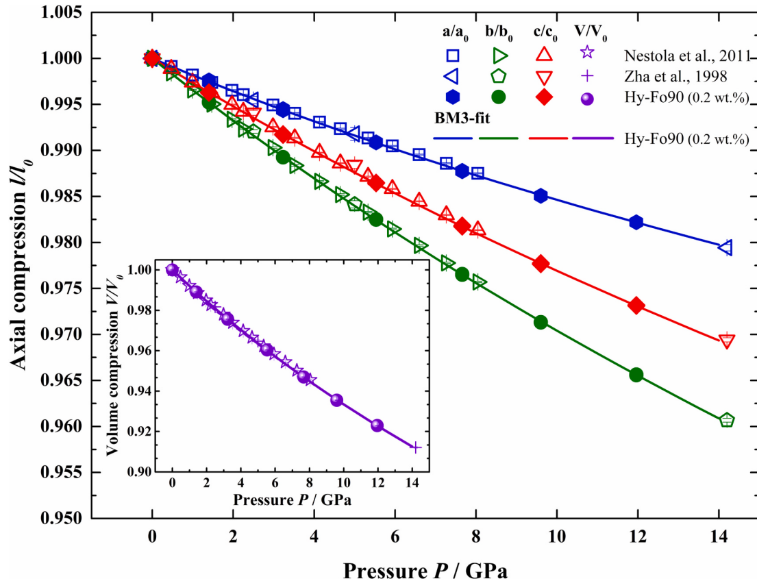
Fig. 2. Unit-cell parameters and unit-cell volumes (inset) of crystals X1 and X2 normalized to their room pressure values; data were fitted with a third-order Birch-Murnaghan EoS using the EoSFit7c program (Angel et al., 2014). Literature data of anhydrous Fo90–92 olivines (Nestola et al., 2011; Zha et al., 1998; Supplementary Table S1) are shown for reference. Note the good agreement between the BM3 fits and relative compression data of hydrous Fo90 olivine and the literature data for the corresponding anhydrous phase.
