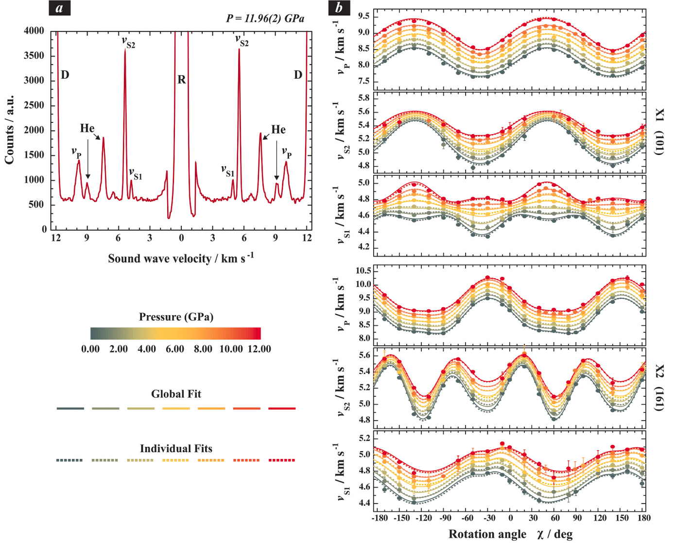
Fig. 3. (a) Selected Brillouin spectrum of crystal X2 (161) at 11.96(2) GPa showing distinct and well-resolved compressional v_P , slow and fast shear v_{S1} and v_{S2} wave velocities peaks, as well as spectral contributions of the diamond anvils (D), pressure medium (He) and elastic scattering (R). (b) Data points (filled symbols) as a function of the rotation angle ( \chi ) for both platelets and dispersion curves obtained from the global fit (solid lines) and individual fits (dashed lines), showing excellent agreement between the two fitting strategies.
