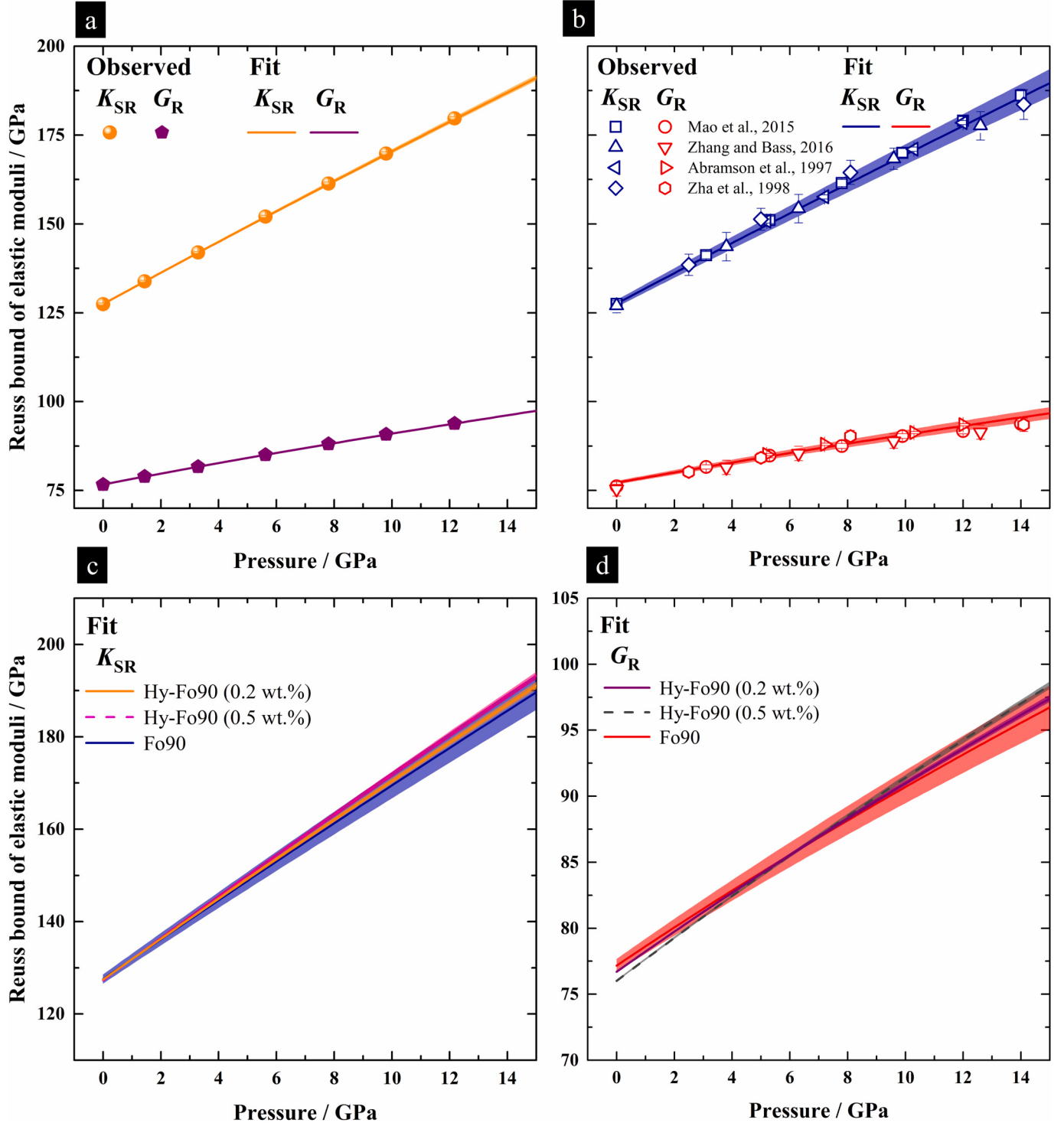
Fig. 5. (a) Variation as a function of pressure of the bulk ( K ) and shear ( G ) moduli of hydrous Fo90 calculated in the Reuss bound from the experimental high-pressure elasticity measurements of this study; the solid line and shaded area are the fit of the experimental data and the associated uncertainty, respectively. (b) Variation as a function of pressure of the bulk ( K ) and shear ( G ) moduli of anhydrous Fo90 calculated in the Reuss bound from previous experimental high-pressure elasticity measurements (Abramson et al., 1997; Mao et al., 2015; Zha et al., 1998; Zhang and Bass, 2016; Supplementary Table S2); the solid line and shaded area are the fit of the experimental data and the associated uncertainty, respectively. (c-d) Superimposition of fit curves for hydrous Fo90 and anhydrous Fo90 olivine; the dashed lines represent a linear extrapolation of the effect of incorporation of 0.5 wt% H 2 O on the elastic properties of Fo90 olivine (see text and Table 4). Uncertainties are calculated by propagating the experimental errors on density and elastic moduli.
