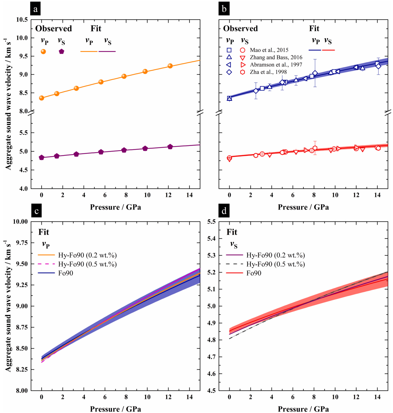
Fig. 6. (a) Variation as a function of pressure of the aggregate compressional and shear wave velocities of hydrous Fo90 calculated from the experimental high-pressure elasticity measurements of this study; the solid line and shaded area the fit of the experimental data and the associated uncertainty, respectively. (b) Variation as a function of pressure of the aggregate compressional and shear wave velocities of anhydrous Fo90 calculated from previous experimental high-pressure elasticity measurements (Abramson et al., 1997; Mao et al., 2015; Zha et al., 1998; Zhang and Bass, 2016; Supplementary Table S2); the solid line and shaded area the fit of the experimental data and the associated uncertainty, respectively. (c-d) Superimposition of fit curves for hydrous Fo90 and anhydrous Fo90 olivine. Uncertainties are calculated by propagating the experimental errors on density and elastic moduli.
