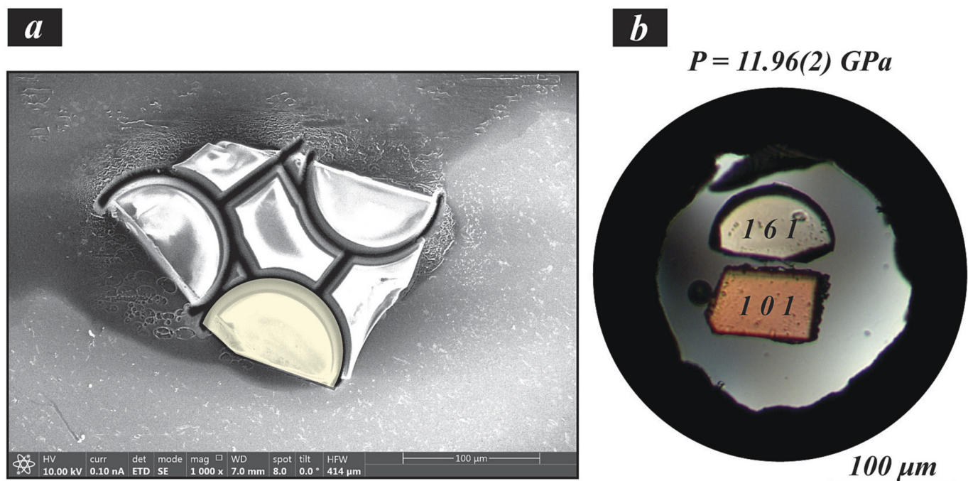
Fig. 1. (a) Secondary electron image of a Fo90 olivine platelet oriented parallel to the (161) plane (crystal X2) after the FIB cutting procedure; a superimposed yellow semicircle denotes the sample that was then loaded in the DAC. (b) Cross-polarized light photomicrographs of platelet X2 (161) and X1 (101) inside the sample chamber of the DAC at high pressure, together with a ruby chip (dark black sphere on the left of 101 platelet).
