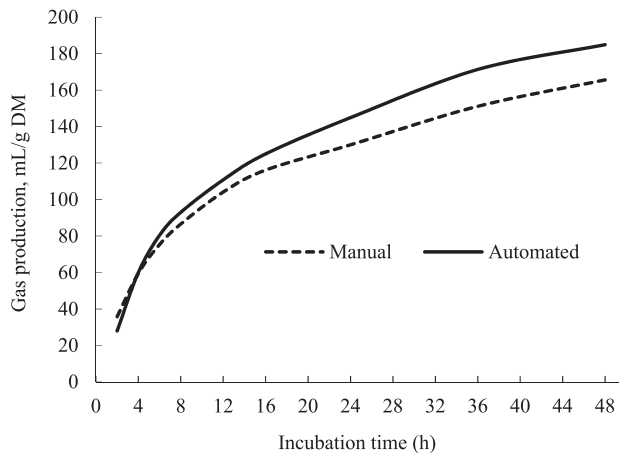
Fig. 2. Gas production measurements determined with automated system (solid lines) or manual technique (dotted lines) where, in two incubation runs six feeds were incubated in four replications for 48 h.
