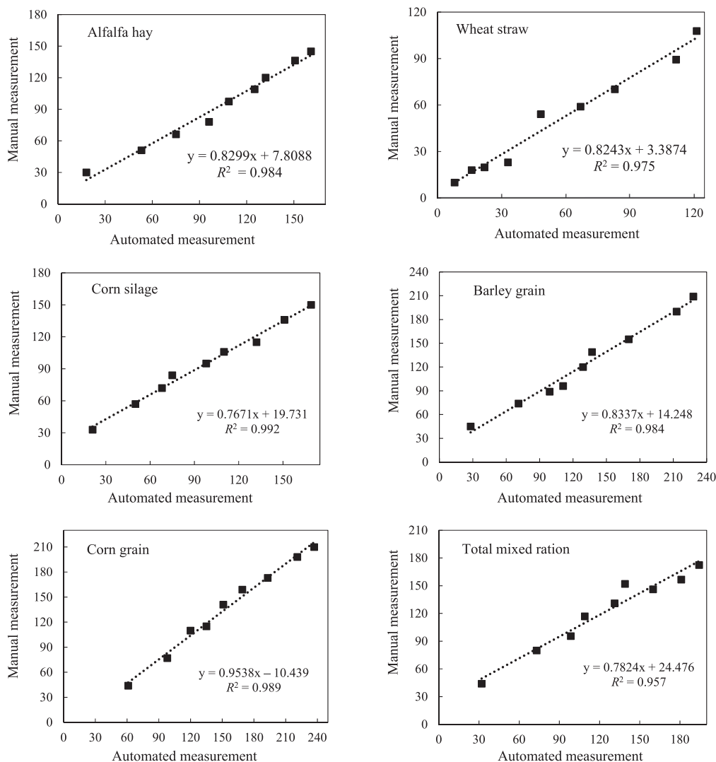
Fig. 3. Relationship between total gas production (mL/g DM) at different incubation times [2, 4, 6, 8, 12, 16, 24, 36, and 48 h] for each feed ingredient measured with automated system or manual technique.
