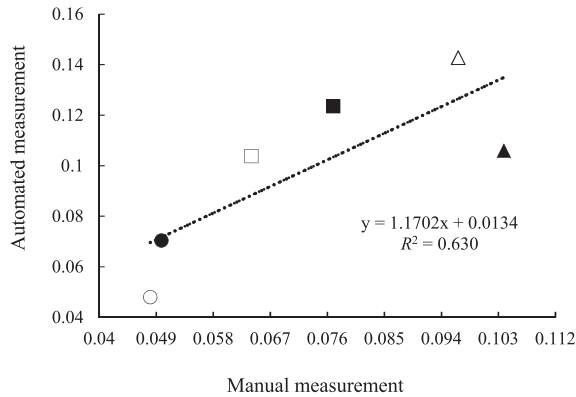
Fig. 4. Relationship between gas production rate constant ( \text{h}^{-1} ) of six experimental feeds (○ wheat straw; ● barley grain; □ corn silage; ■ corn grain; △ total mixed ration; ▲ alfalfa hay) measured with automated or manual system.
