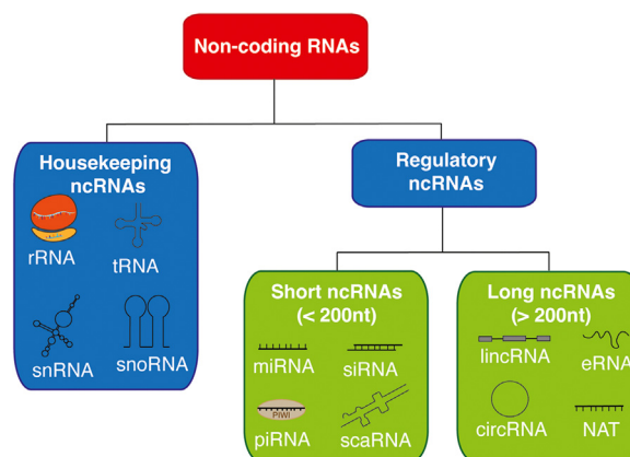
Fig 2. Classification of noncoding RNA. Noncoding RNA can be divided into 2 groups: housekeeping and regulatory ncRNA. The regulatory ncRNA can also be divided into 2 groups based on their size (long and short ncRNA). (For interpretation of the references to color in this figure legend, the reader is referred to the Web version of this article.)
