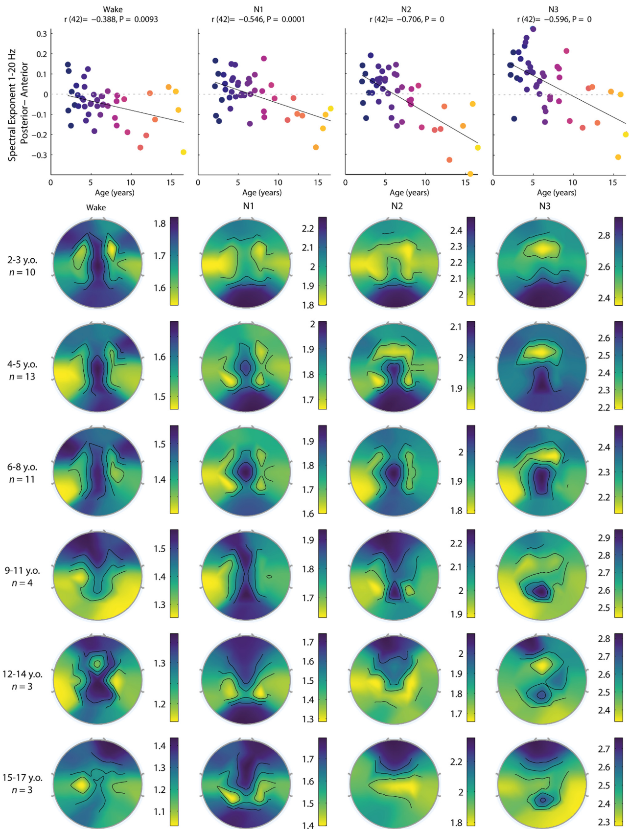
Fig. 4. Throughout vigilance stages, the posterior-to-anterior difference of the spectral exponent negatively correlates with age and the location with higher values of spectral exponent migrates from posterior to anterior regions from childhood to adolescence. Correlation between age and posterior-to-anterior difference of spectral exponent in wakefulness and sleep stages. Color coded topographies display the distribution of spectral exponent over the scalp across vigilance stages, averaged within groups of subjects of different age ranges. The region with steeper spectral exponent is color coded in blue, within each topography.
