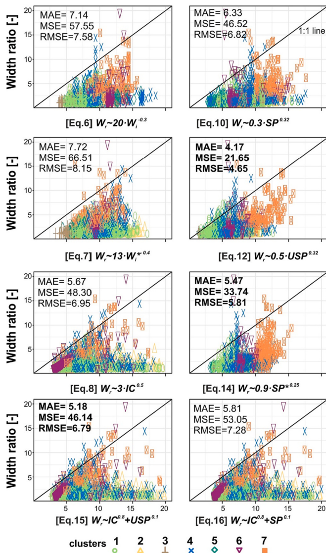
Fig. 11. Observed width ratio ( W_r ) versus estimated values obtained by applying the upper envelope equations shown in Table 6, for all data coloured by clusters. The black line is the 1:1 line. MAE: mean absolute error; MSE: mean squared error; RMSE: root mean squared error. W_i : initial channel width; W_i^* : normalized width; IC: confinement index; USP: unit flood stream power; and SP^* : normalized stream power. Better performance shown in bold.
