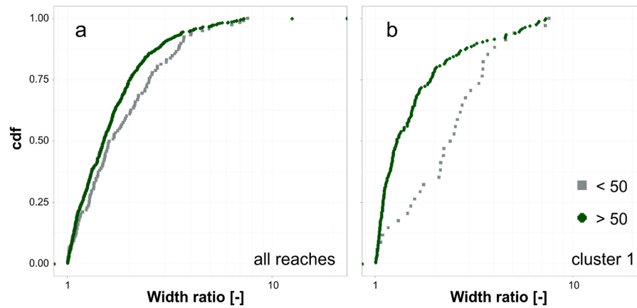
Fig. 8. Cumulative distribution functions (cdf) of width ratio for all reaches grouped by forested channel length class (> or < 50 %) and cluster 1.
