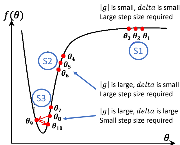
FIGURE 4: A common situation in optimization that illustrates the significance of adaptive parameter updates in the optimization process [49].
