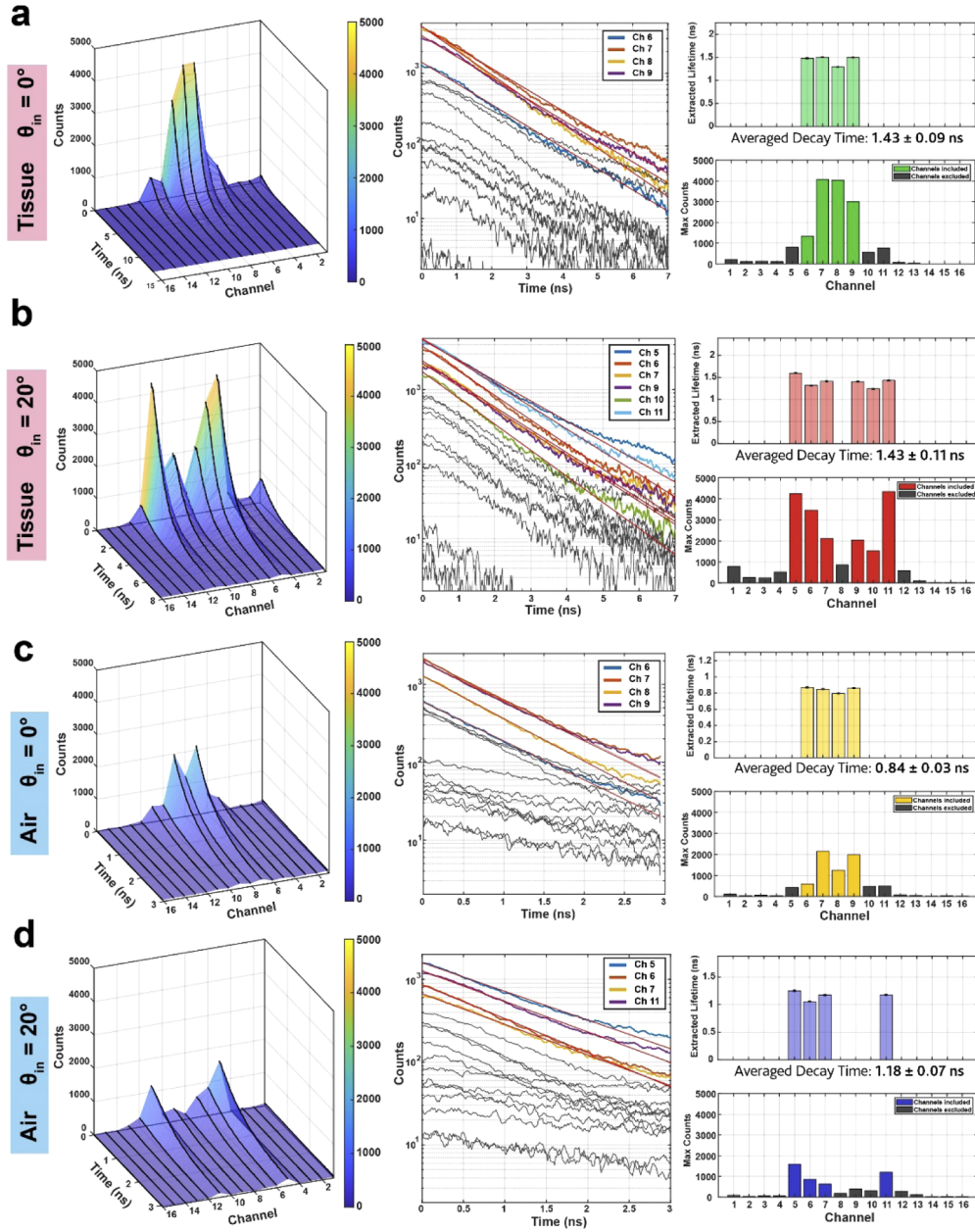
Fig. 5. (a-b) Results of the analysis for DR-FLiP measurements with the TF (Sample S2, taper angle 3.7^\circ ) implanted in a 300\text{ }\mu\text{m} -thick coronal brain slice from a (Thy1-GCaMP6s) GP4.12Dkim/J mouse, \theta_{in} = 0^\circ , and \theta_{in} = 20^\circ . Left column is the decay map for all the channels of the array. Center column shows the results of the fitting for the decay tracks over threshold, logarithmic scale. Tracks under threshold are shown in gray, and are excluded from the evaluation of the lifetime \tau . On right column are reported the extracted lifetimes, and the maximum counts per channel. (c-d) Same analysis for the AF of the fiber, for \theta_{in} = 0^\circ , and \theta_{in} = 20^\circ .
