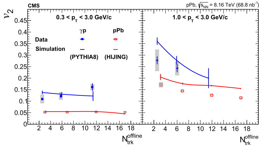
Fig. 4. Single-particle azimuthal anisotropy v_2 versus N_{\text{trk}}^{\text{offline}} for \gamma p -enhanced and pPb samples in two p_T -regions. Systematic uncertainties are shown by the shaded bars in the two panels. Predictions from the PYTHIA8 and HIJING generators are shown for the \gamma p and MB pPb samples respectively. For the \gamma p events, same N_{\text{trk}}^{\text{offline}} bin arrangement as in Fig. 3 is kept while for pPb the bins [2, 5), [5, 10), [10, 15) and [15, 20) are used.
