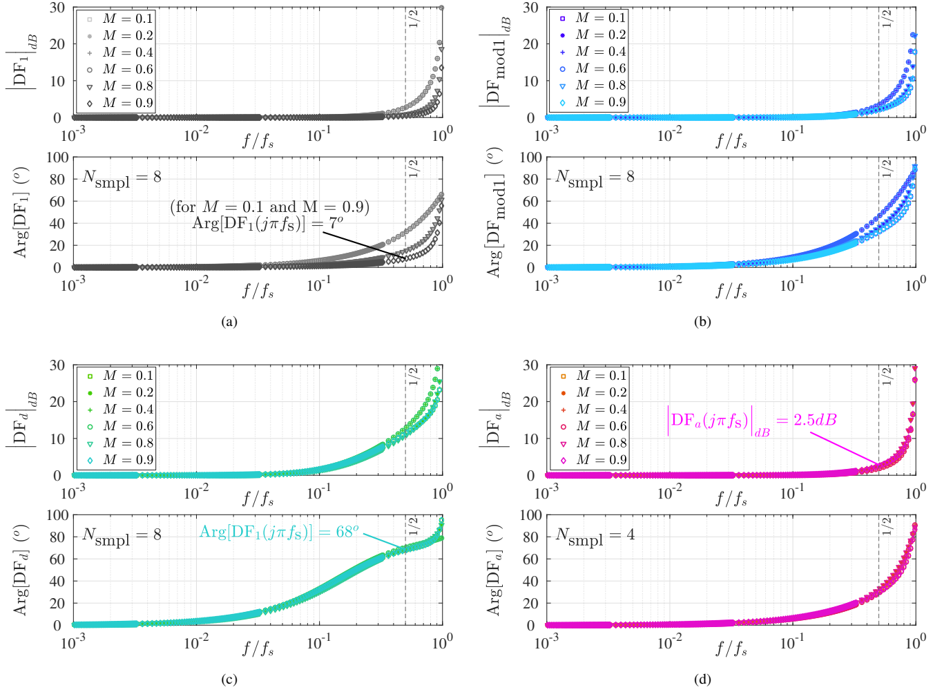
Fig. 4: Bode plot of the analytical small-signal models of (a) DF_1(s) and (b) DF_{\text{mod1}}(s) proposed respectively in [26] and [28] for N_{\text{smpl}} = 8 , and Bode plot of (c) DF_d(s) ( N_{\text{smpl}} = 8 ) and (d) DF_a(s) ( N_{\text{smpl}} = 4 ).
