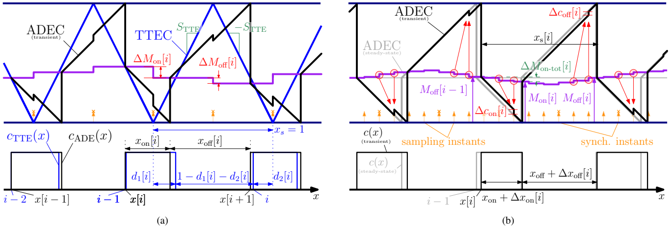
Fig. 1: (a) Exemplified time operation of (blue lines) TTEC and (black lines) ADEC-based double-sampling DPWMs and corresponding control signals (bottom). (b) Exemplified time operation of the multi-sampling ADE-DPWM for N_{smpl} = 8 . Gray lines represent the steady-state operation.
