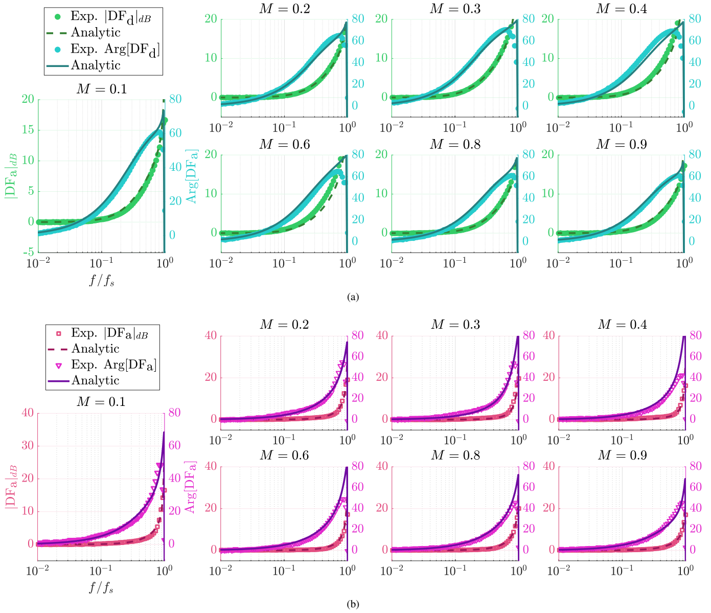
Fig. 7: Bode-plot comparison of (a) DF_d(s) and (b) DF_a(s) vs the corresponding experimental transfer function measurements.
