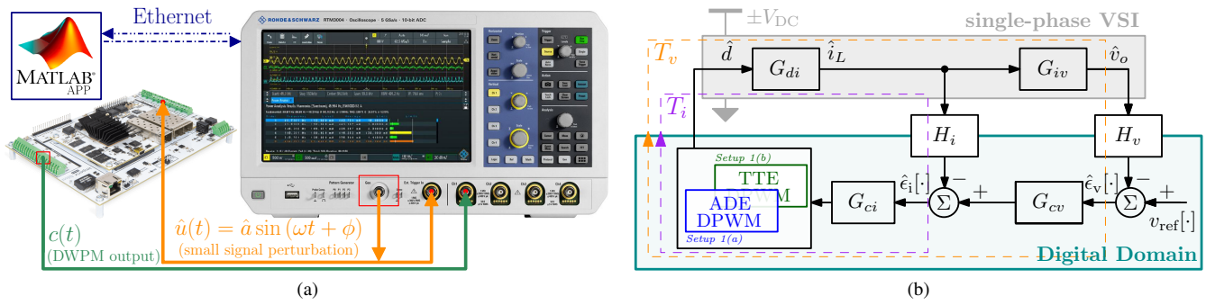
Fig. 6: (a) Experimental setup for the small-signal transfer function measurements. (b) Block diagram representation of the selected case-study.
