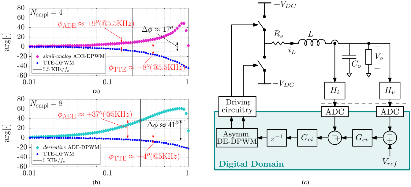
Fig. 8: Comparison between the experimental phase response of (a) the simil-analog ADE-DPWM ( N_{\text{smpl}} = 4 ) vs the TTE-DPWM ( N_{\text{smpl}} = 4 ) and (b) the derivative ADE-DPWM ( N_{\text{smpl}} = 8 ) vs the TTE-DPWM ( N_{\text{smpl}} = 8 ). Horizontal axes represent the normalized frequency (i.e., f/f_s ). (c) Circuit and block diagram representation of the output voltage controlled single-phase voltage-source inverter used in the experimental measurements in Sec. VI.
