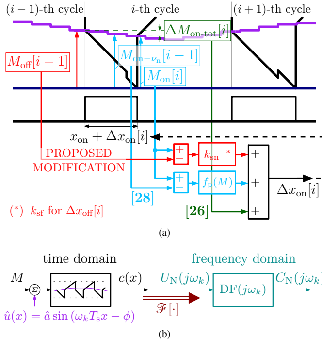
Fig. 2: (a) Evolution of multi-sampling ADE-DPWM architectures. The green patch represents the structure in [26], the light-blue path the modification introduced in [28]. The red one represents the additional path proposed in this manuscript. (b) Graphical representation and notation for the small signal analysis of the ADE-DPWM.
