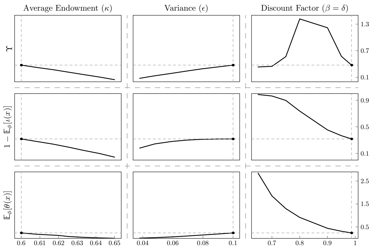
Figure C.1. — Comparative Statics on the Martin-Ross Bound \Upsilon , the Expected Insurance Coefficient and the Expected Consumption Equivalent Welfare Change.
