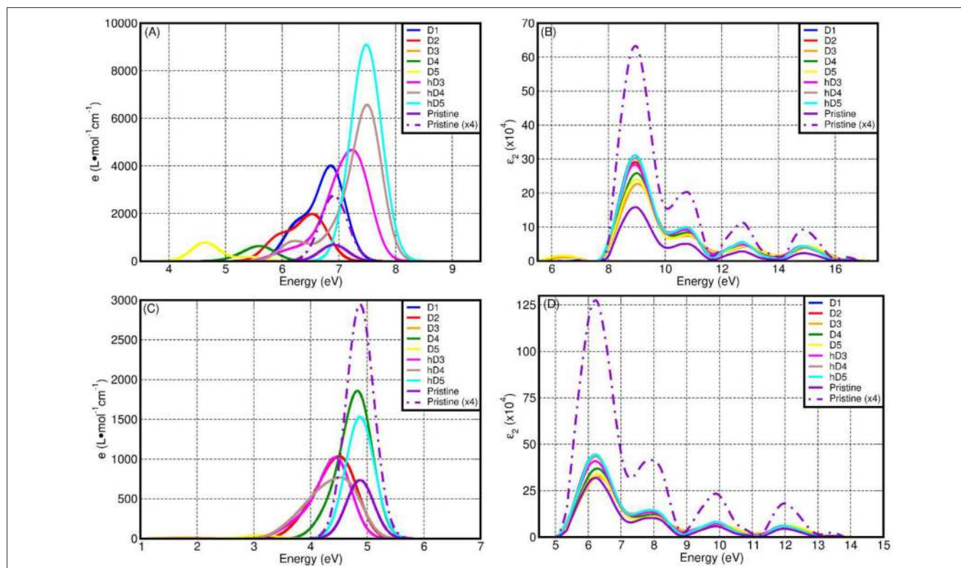
FIGURE 8 | Computed LR-TDA-TDDFT optical spectra at PBE0-TC-LRC (A) and PBE (C) level of theory for all the systems considered, together with the corresponding FGR spectra, also at PBE0-TH-LRC (B) and PBE (D) level. Owing to the substantially lower computed absorbance, the D3 traces in (A,C) cannot be resolved for the adopted scale of the y-axis.
