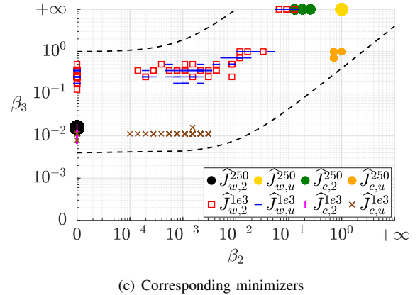
Fig. 1: (a): comparison between the Kalman-filter-based oracle performance J_{OR} and the minimum cost realizations \hat{J}_{n_s, rg}^{N_{data}} for \Sigma_L over 100 Monte Carlo runs; (b): Optimal performance under the constraint \beta_2 = 0 ; (c): distribution of the corresponding minimizers (\beta_2^*, \beta_3^*) .
