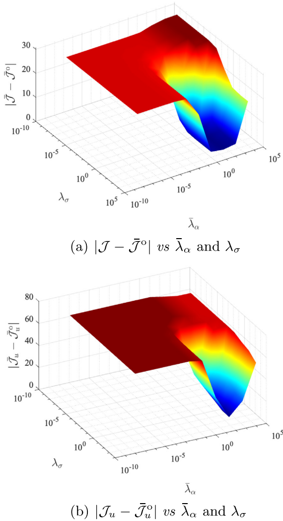
Fig. 9. Closed-loop validation tests ( \overline{\text{SNR}} = 18 dB): absolute differences between the performance indexes attained with Berberich et al. (2020) and the average values of those associated with the noisy oracle MPC vs. penalties \bar{\lambda}_\alpha = \lambda_\alpha \bar{\varepsilon} and \lambda_\sigma over 30 Monte Carlo predictors.
