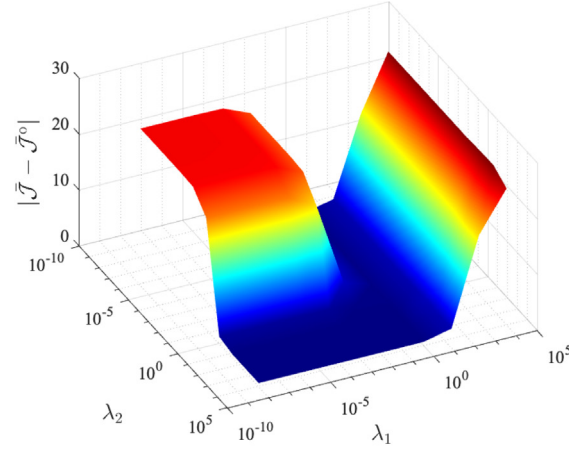
(a) |\mathcal{J} - \bar{\mathcal{J}}^o| vs \lambda_1 and \lambda_2
