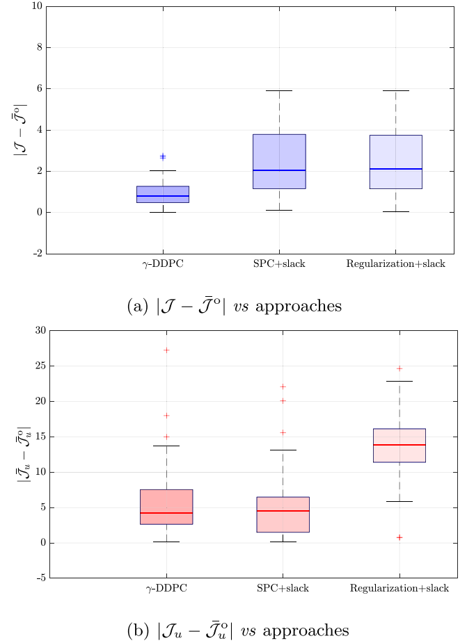
Fig. 10. Closed-loop validation tests ( \overline{\text{SNR}} = 18 dB): absolute differences between the average performance indexes attained with the noisy oracle MPC and \mathcal{J} and \mathcal{J}_u obtained with \gamma -DDPC, and the SPC+slack scheme in (30) and the regularized approach with slack in (31) with the best tuning over 30 Monte Carlo predictors..
