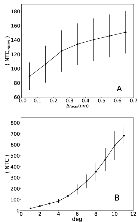
Fig. 5. A: Average value of \text{NTC}_{\text{mean}}(\tau) as a function of different intervals of the mobility \Delta r_{\max}(\tau_4) at 230 K. B: Average value of NTC as a function of different values of the degree centrality at 230 K. In A and B, the error bars are obtained considering the standard deviation.
