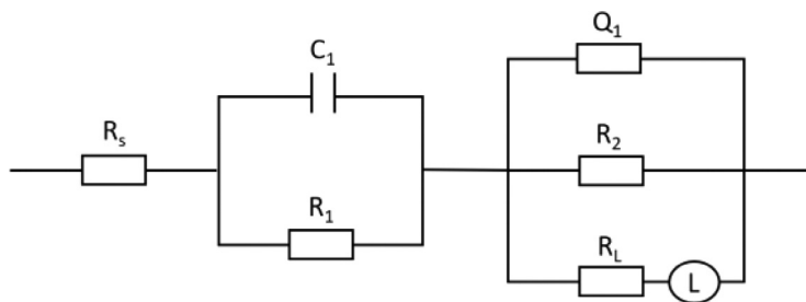
Fig. 13. Equivalent Circuit for EIS spectra.
