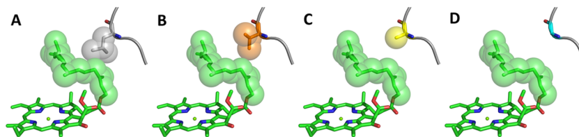
Figure 5. Comparison between Lv-wt (A), Lv-L91V (B), L91A (C), and L91G (D) (with residue 91 in gray, orange, yellow, and light blue, respectively). The structure of Lv-wt 15 is shown, with the polypeptide chain in gray cartoons and the Chls a in green. The mutations have been introduced in silico with PyMOL Mutagenesis Tool. Phytyls and the side chains of residue 91 have been highlighted in spheres.
