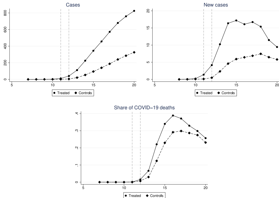
Fig. 5. Weekly values of COVID-19 cases, COVID-19 new cases, COVID-19 deaths, all deaths, and share of COVID-19 deaths on all deaths.
