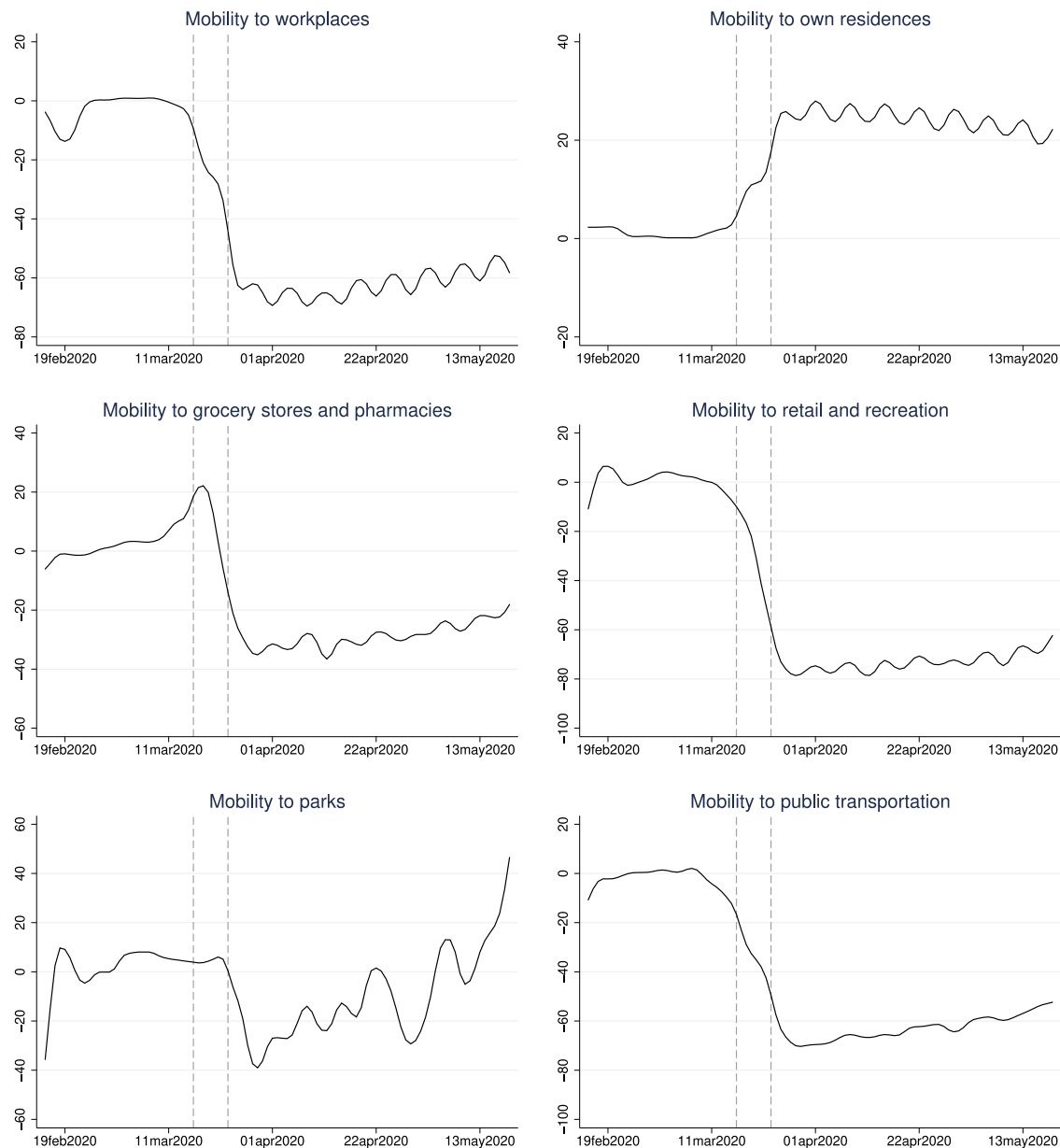
Fig. 4. Mobility trends during the period 15/2 - 19/5 of 2020.
