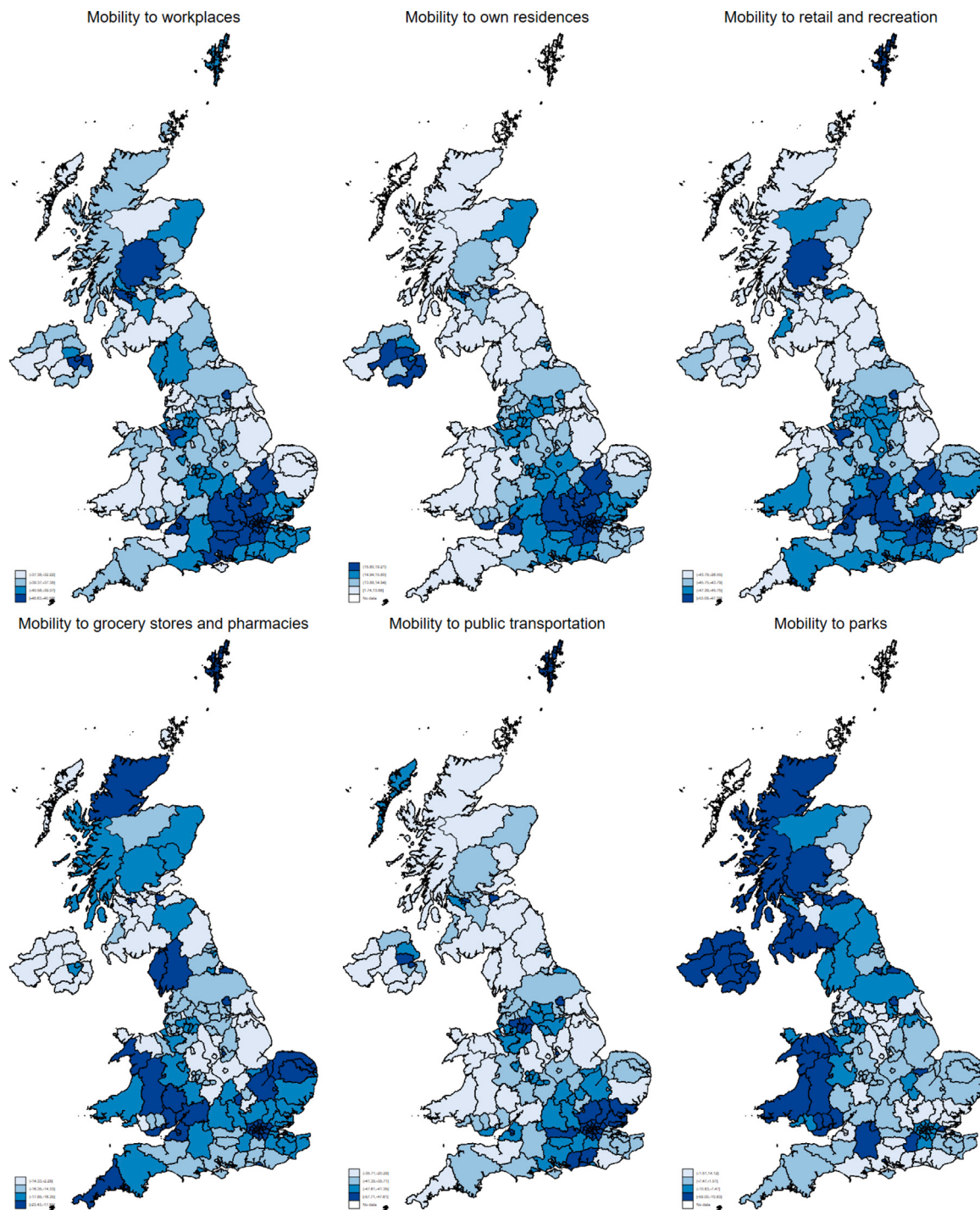
Fig. 2. Territorial distribution of changes in mobility. Average values for the period 15/2 - 19/5 of 2020.
