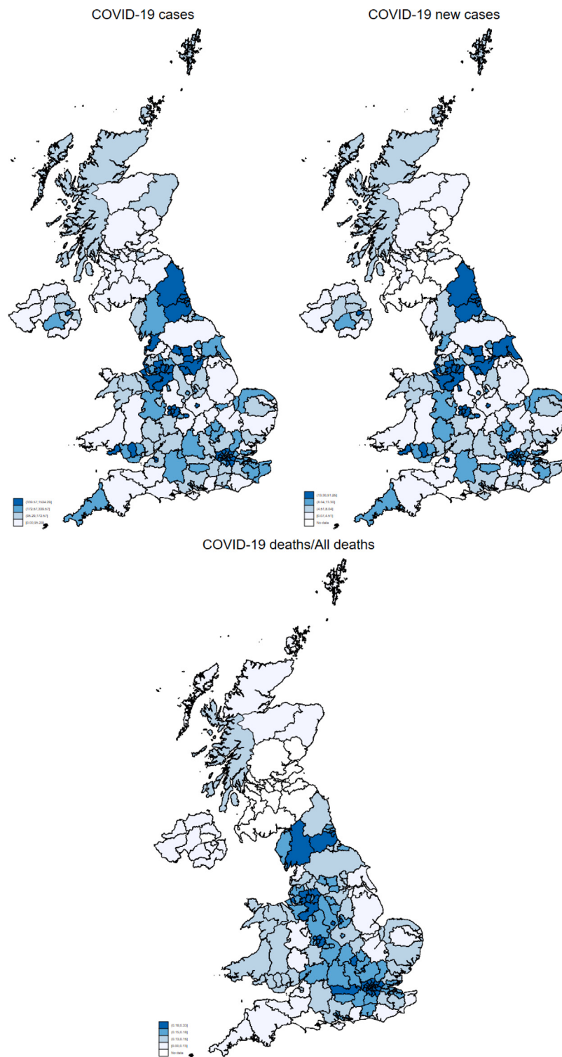
Fig. 3. Geographical variability for the ratio between COVID-19 deaths and deaths for other causes.
