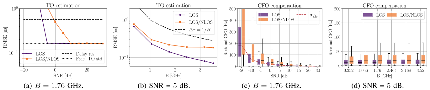
Fig. 6. Simulation results for TO estimation RMSE (a-b) and CFO compensation error distribution (c-d), varying the SNR and the TX signal bandwidth. We report the results for LOS and intermittent LOS/NLOS conditions.
