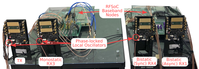
Fig. 8. Testbed components.
