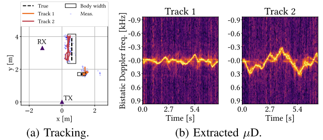
Fig. 14. \mu\text{D} extracted in a multitarget scenario.
