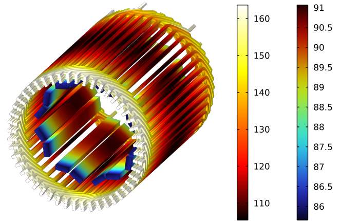
Fig. 8: Temperature distribution on windings and magnets. Values are in °C.
