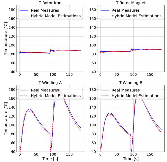
Fig. 13: Peak Torque Validation Set. Note that, for the sake of conciseness, 2 different tests are reported in this figure.
