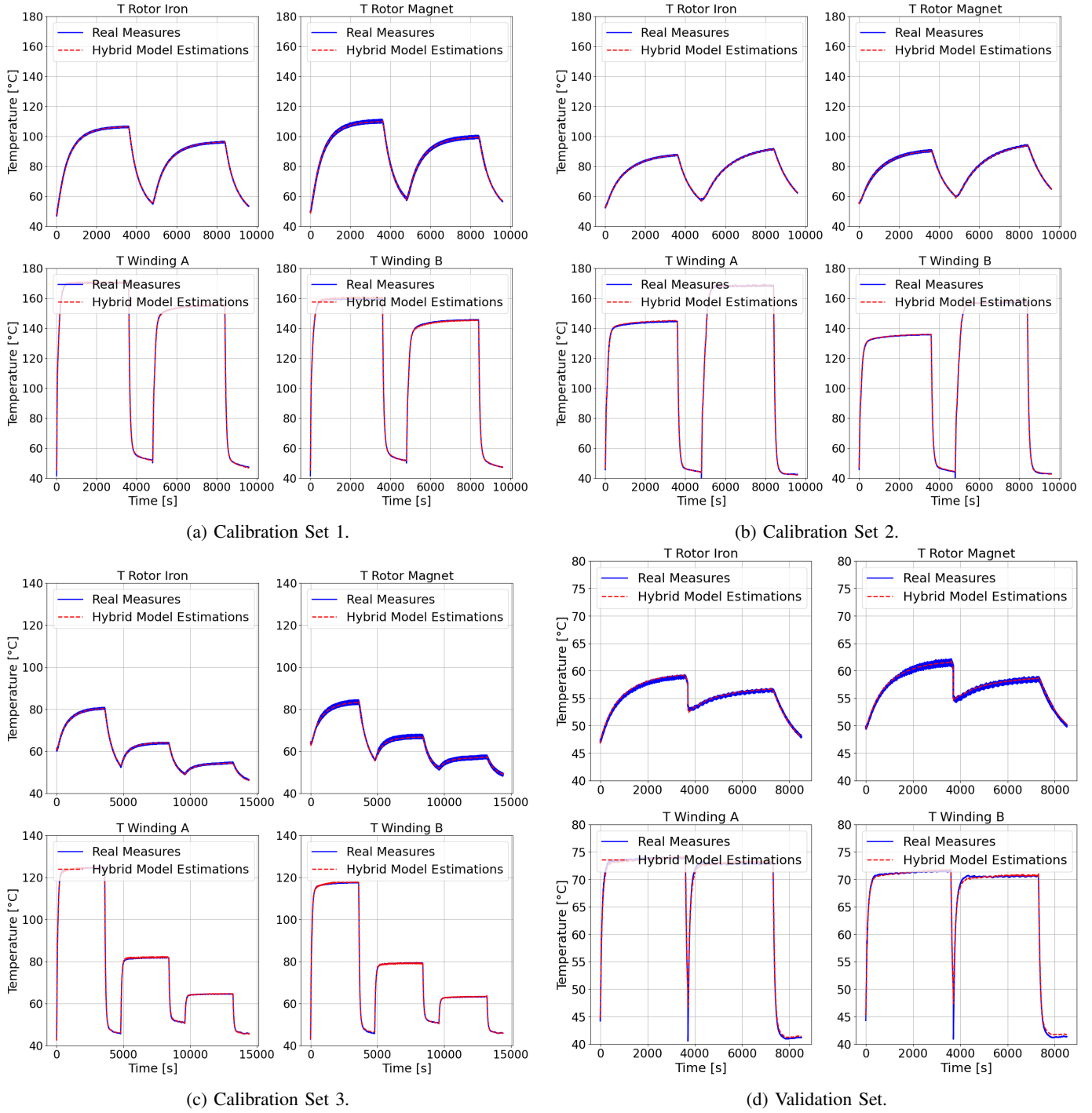
Fig. 11: Calibration and validation sets.
