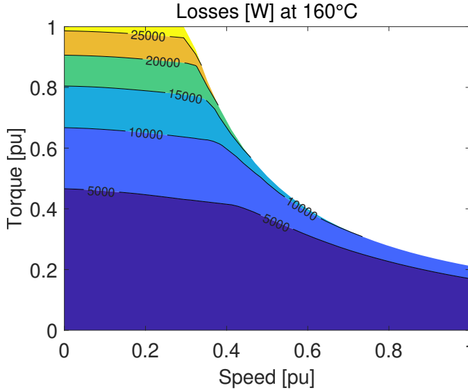
Fig. 6: Total losses at 160°C.
