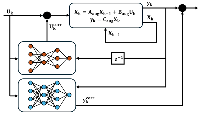
Fig. 9: Hybrid Model Architecture (Physics Based and AI Data-Driven Based).
