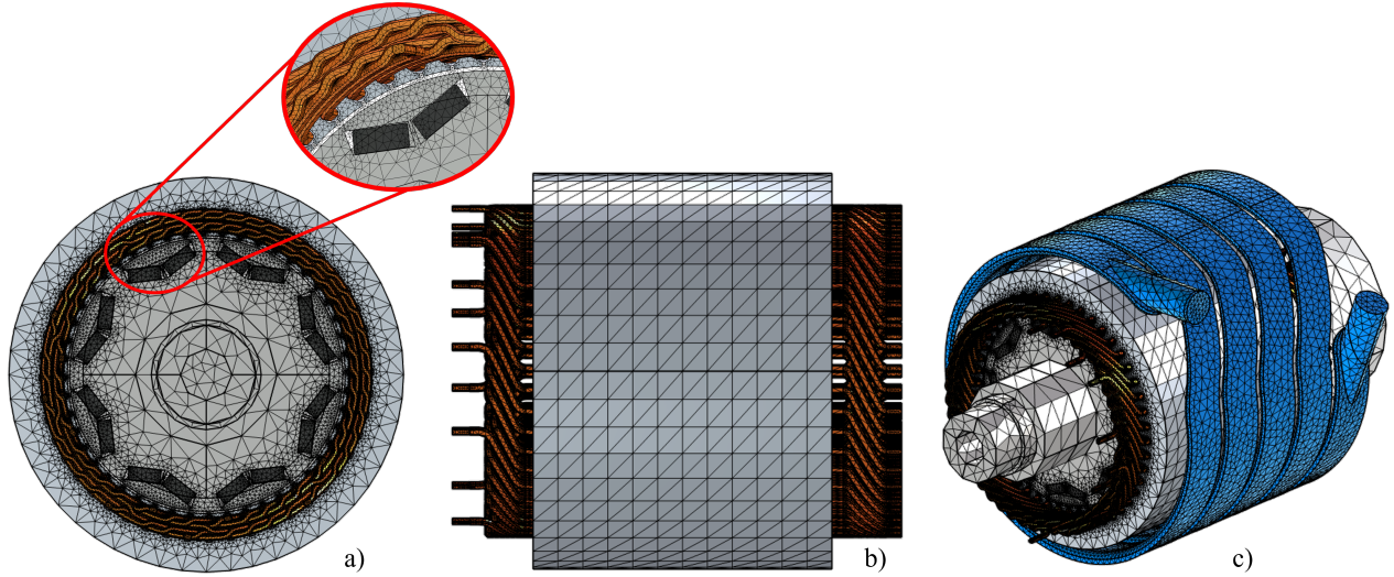
Fig. 7: Mesh of the the 3D FEM model. a) Frontal view. b) axial view. c) 3D view.
