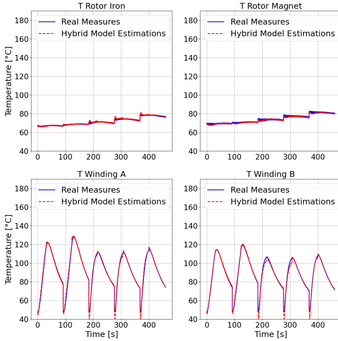
Fig. 12: Peak Torque Calibration Set. Note that, for the sake of conciseness, 5 different tests are reported in this figure.
