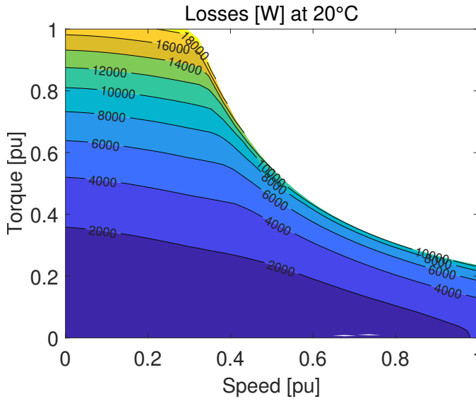
Fig. 5: Total losses at 20°C.
