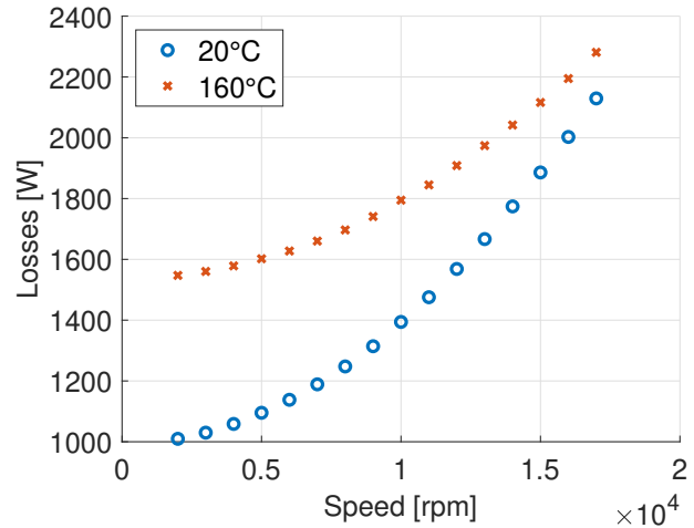
Fig. 4: Winding losses vs speed at 20°C and 160°C.
