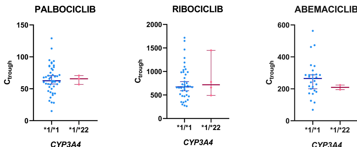
Fig. 2. Association between CYP3A4 *22 polymorphism and C_{trough} of each CDKi. Box plots depict the median (horizontal bar) and 95% Confidence Interval (CI). The dots represent individual concentration values.
