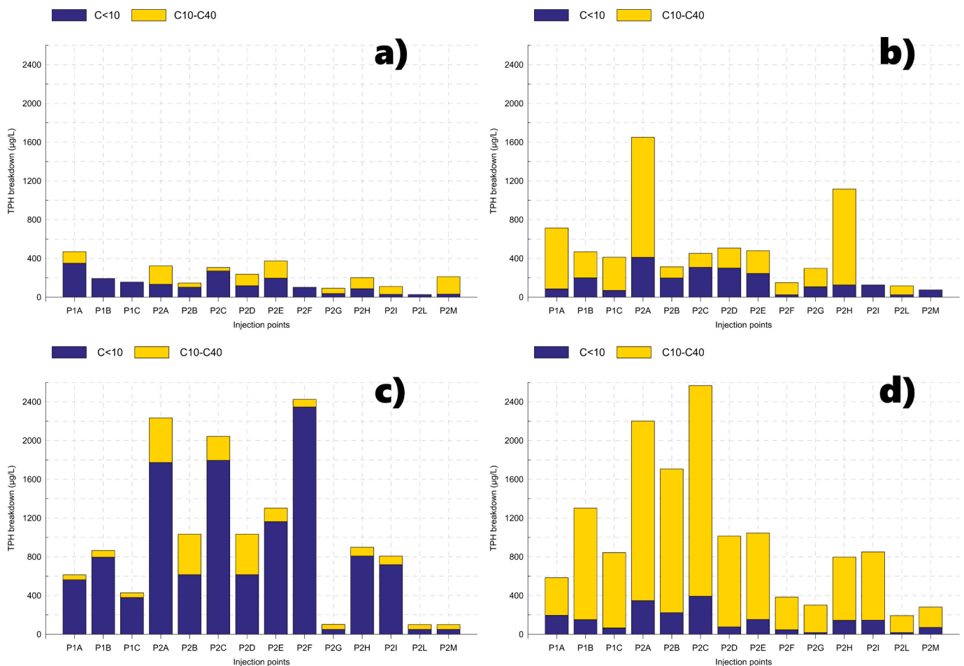
Fig. 6. Concentrations of light hydrocarbon fractions ( C < 10 ) and heavy fractions (C10-C40) measured in the 14 reagent introduction wells along line CD, before (a), one (b), two (c), and three (d) months after the injection activities.
