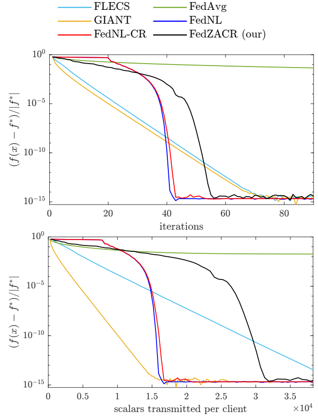
FIGURE 4: Training loss of standard logistic regression: unfair comparison between the zeroth-order FedZACR versus other federated algorithms that make use of the exact derivatives. While FedZACR is clearly disadvantaged, its performance is comparable to second-order state-of-the-art algorithms.
