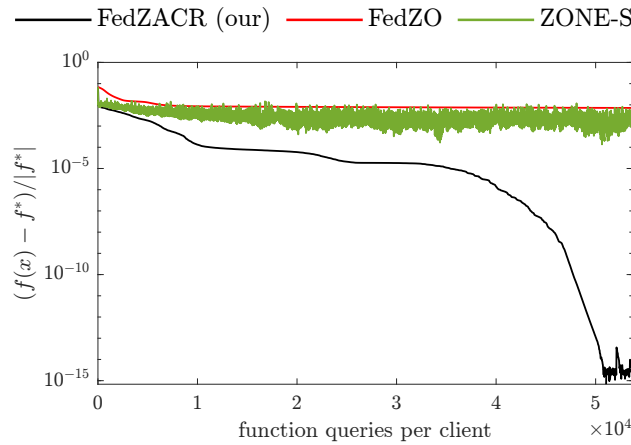
FIGURE 5: Function value suboptimality of zeroth-order linear regression using a non-convex loss. We compare FedZACR to other federated zeroth-order algorithms.
