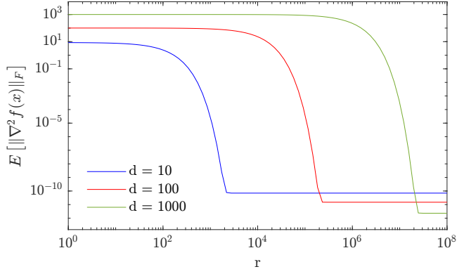
FIGURE 1: Visual representation of the bound provided by Lemma 3, setting \hat{H}^0 = 0_d , L_3 = 0.05 , \mu = 10^{-4} . The Hessian matrices are random matrices whose elements are i.i.d. \sim \mathcal{N}(0, 1) .
