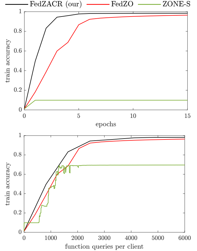
FIGURE 6: Training accuracy achieved while fine-tuning a black-box neural network on a classification task. FedZACR is compared with other federated zeroth-order algorithms for non-convex optimization.
