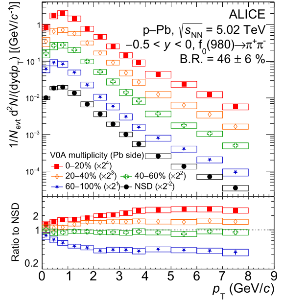
Fig. 2. Transverse momentum spectra of f_0(980) in p-Pb collisions at \sqrt{s_{\text{NN}}} = 5.02 TeV for different multiplicity classes, which are scaled for visibility. Statistical and systematic uncertainties are shown as error bars and boxes, respectively. The normalization uncertainty of 13% due to the uncertainty of the B.R. is not shown in the figure. The lower panel shows the ratios of the spectra in multiplicity classes to the NSD spectrum.
