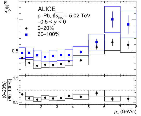
Fig. 5. The particle yield ratio of f_0(980) to K^*(892)^0 as a function of p_T in high-multiplicity (circles) and low-multiplicity (squares) p-Pb collisions at \sqrt{s_{NN}} = 5.02 TeV. The lower panel shows the double ratio of high-multiplicity to low-multiplicity f_0(980)/K^*(892)^0 . V0A is utilized to categorize events based on their multiplicity.
