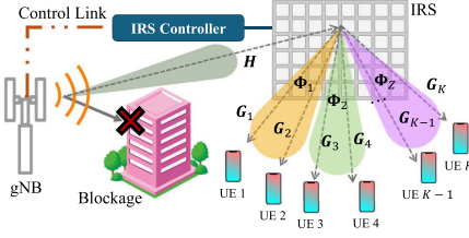
Fig. 1. OFDMA scheduling for IRS-assisted multi-user equipment (UE) communication.
