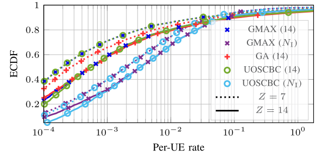
Fig. 4. ECDF of the per-user rate, for K = 90 UEs, F = 5 carrier frequencies, and Z \in \{7, 14\} . Between brackets is the number b_q of bits in the codebook.
