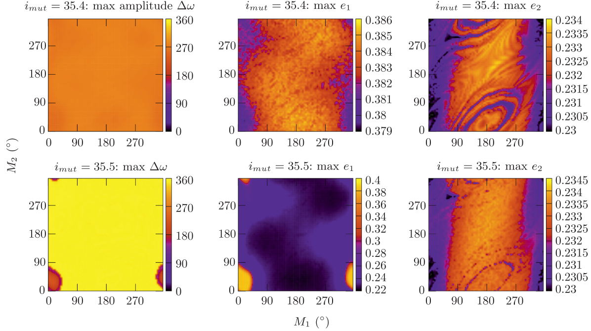
Fig. 5. Results obtained in the parameter space of the mean anomalies (M_1, M_2) for a fixed value of i = 80^\circ and for i_{mut} = 35.4^\circ (top row) and i_{mut} = 35.5^\circ (bottom row). From left to right: the maximal amplitude of the libration of the angle \Delta\omega , the maximal value of the eccentricity of the inner planet e_1 , and of the outer planet e_2 .
