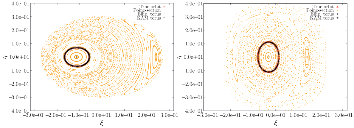
Fig. 3. Poincaré section of the system HD 4732, considering \eta_2 = 0 . On the left, the case relative to the parameters i = 90^{\circ} and i_{mut} = 15^{\circ} . On the right, the case for i = 74^{\circ} and i_{mut} = 37^{\circ} .
