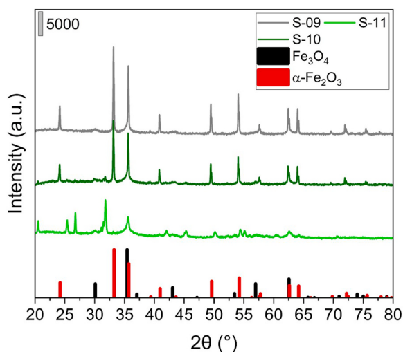
Fig. 5. XRD patterns of samples obtained in mixed solvents/PEG400 50/50 environment, maintaining constant the volume of mixed PEG400, and varying the water/2-pr. ratio, namely: S-09 (75/25, grey), S-10 (50/50, olive), and S-11 (25/75, green). XRD reference patterns: magnetite (01–074–0748, \text{Fe}_3\text{O}_4 , black), and hematite (01–089–8104, \alpha\text{-Fe}_2\text{O}_3 , red).
