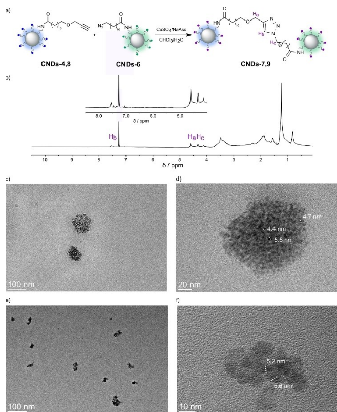
Figure 4. a) General scheme for the click reaction between CNDs-4,8 and CNDs-6 . The colored labels correspond to the depicted functionalities. Conditions: CNDs-4,8 (5–10 mg), CNDs-6 (15 mg), CuSO 4 ·5H 2 O (0.005 mmol), NaAsc (0.01 mmol), CHCl 3 (1 mL), H 2 O (1 mL), 24 h. b) CNDs-7 , ^1\text{H} NMR (CDCl 3 , 400 MHz, rt). c–d) TEM images of CNDs-7 . e–f) TEM images of CNDs-9 .
