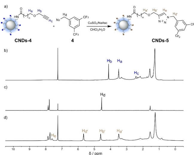
Figure 3. a) General scheme for the click reaction between CNDs-4 and 4 . The colored labels correspond to the depicted functionalities. Conditions: CNDs-4 (15 mg), 4 (0.2 mmol), \text{CuSO}_4 \cdot 5\text{H}_2\text{O} (0.02 mmol), NaAsc (0.04 mmol), \text{CHCl}_3 (1 mL), \text{H}_2\text{O} (1 mL), 24 h. b–d) ^1\text{H} NMR ( \text{CDCl}_3 , 400 MHz, rt) of CNDs-4 , 4 , CNDs-5 .
