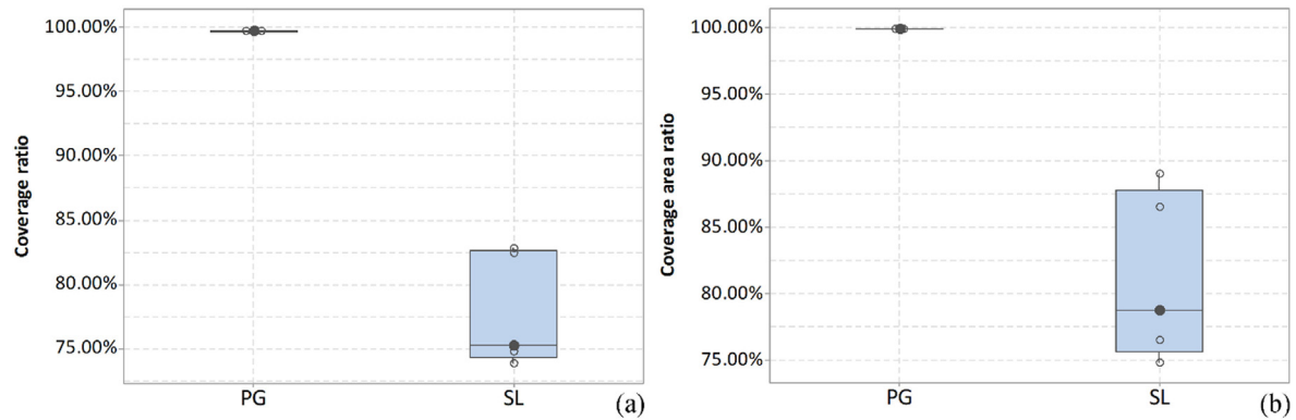
Fig. 4. Indicators of part coverage (boxplots from five measurement repeats): (a) coverage ratio, and (b) coverage area ratio.
