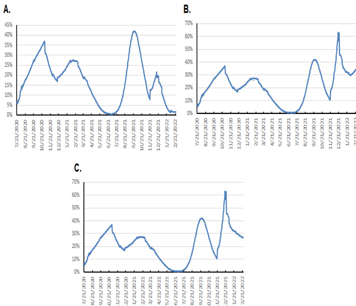
Fig. 1. Daily dynamics of SARS-CoV-2 infection, July 21, 2020 to February 21, 2022.
