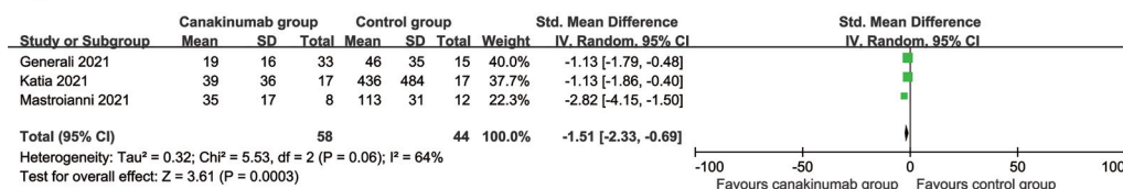
Fig. 1. A Association between canakinumab treatment and mortality, Fig. 1B. Association between canakinumab treatment and developing severe COVID-19, Fig. 1C Association between canakinumab treatment and CRP levels.
