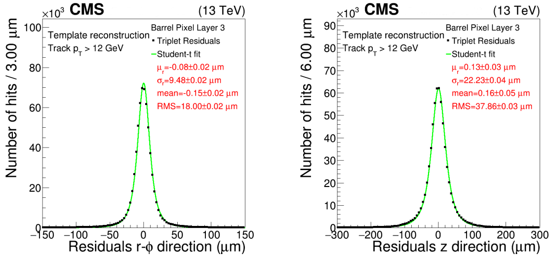
Figure 48. Pixel hit residuals for BPIX L3 in r\phi (left) and z direction (right). The data correspond to an integrated luminosity of about 75 fb -1 .
