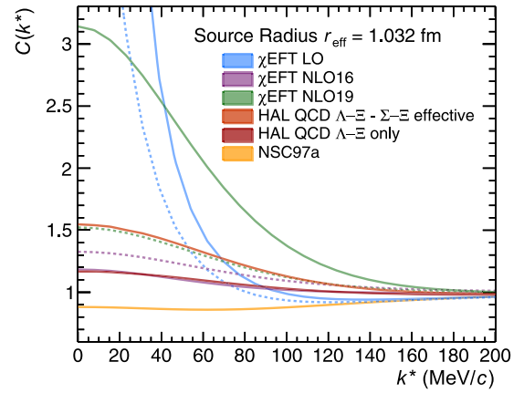
Fig. 1. Theoretical \Lambda-\Xi^- correlation functions from predictions ([2,11,12,16]) evaluated for the experimental source radius. See text for details. In the case of the LO and NLO \chi EFT potentials the solid (dotted) lines correspond to the lowest (highest) cutoff [11,16].
