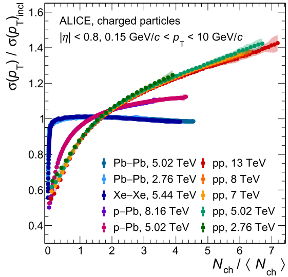
Fig. 1. Relative standard deviation of the charged-particle transverse momentum spectrum as a function of the relative charged-particle multiplicity N_{\text{ch}}/\langle N_{\text{ch}} \rangle in pp, p–Pb, Xe–Xe, and Pb–Pb collisions at various centre-of-mass energies per nucleon pair. The standard deviation \sigma(p_T) for each multiplicity is shown relative to the multiplicity-inclusive value \sigma(p_T)_{\text{incl}} . Statistical and systematic uncertainties are shown as bars and semi-transparent bands, respectively.
