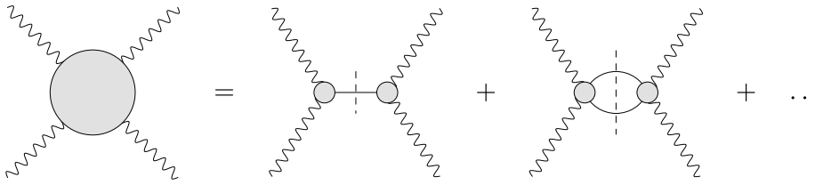
Fig. 51. Intermediate states in the direct channel for HLbL scattering: one- and two-particle cut. The gray blobs denote hadronic amplitudes involving \gamma^* \gamma^* \gamma^{(*)} . Source: Reprinted from Ref. [20].
