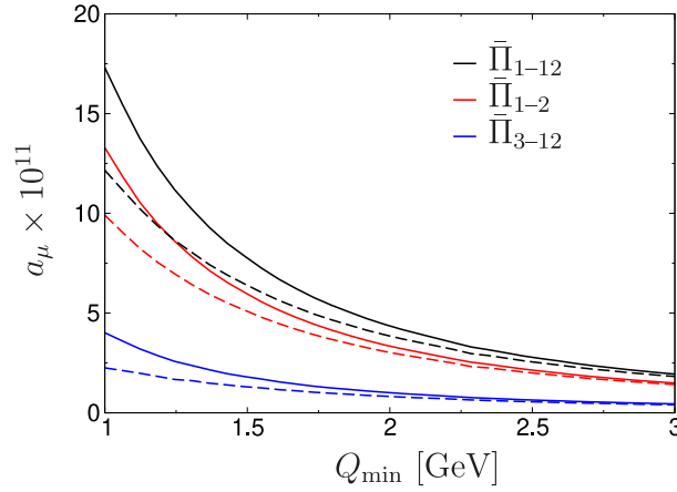
Fig. 70. Contribution of the pQCD quark loop to a_\mu for Q_i \geq Q_{\min} . Solid lines for vanishing quark masses, dashed lines for m_q = 0.3 GeV. The total contribution from \tilde{\Pi}_{1-12} is shown in black, together with the partial ones from \tilde{\Pi}_{1-2} (red) and \tilde{\Pi}_{3-12} (blue).
