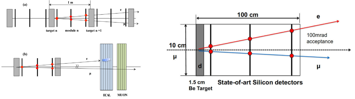
Fig. 34. Left: design of the baseline detector concept. Right: single station.
