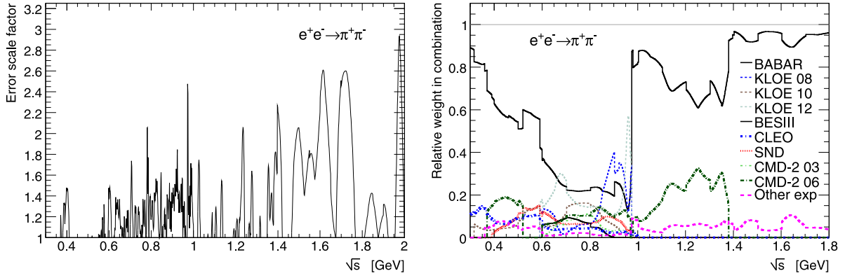
Fig. 23. Left: Rescaling factor accounting for inconsistencies among experiments versus \sqrt{s} . Right: Relative averaging weights per experiment versus \sqrt{s} (see text).
