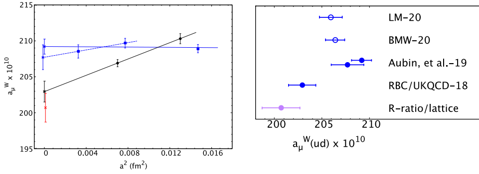
Fig. 47. (Left) Continuum limit of the intermediate window a_\mu^W(ud) ( \Delta = 0.15 \text{ fm} , t_0 = 0.4 \text{ fm} , t_1 = 1 \text{ fm} ) for DW (circles) and HISQ (squares) fermions. Lines denote fits linear in a^2 for the a \rightarrow 0 limit (bursts). The R-ratio result (cross, Ref. [445]) is also shown. It corresponds to the difference of the total R-ratio window result based on Ref. [3] and the sum of all but the isospin-symmetric light-quark lattice results of Ref. [11]. Finite-volume (DWF and HISQ) and taste-breaking (HISQ) corrections are included to NLO in ChPT. Lattice spacing uncertainties, added in quadrature with statistical errors, are also included. Plot reproduced from Ref. [16]. (Right) Comparison of a_\mu^W(ud) results after continuum and infinite-volume extrapolation (blue circles). The RBC/UKQCD-18 result [11] is based on 2+1 flavors of DW fermions. All other lattice results are based on 2+1+1 flavors of HISQ fermions [16,396,446]. Both extrapolations for HISQ shown in the left panel are reproduced in the right panel as well for comparison. The DW and R-ratio results are the same as shown in the left panel.
