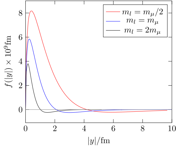
Fig. 80. Integrant of the lepton loop for different loop-particle masses m_l . Source: Reprinted from Ref. [724].
