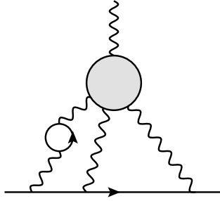
Fig. 72. HLbL scattering combined with lepton vacuum polarization. Diagrams where the lepton loop is inserted into the other photon propagators are not shown.
