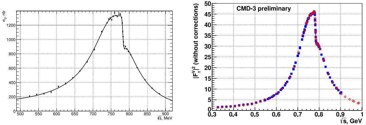
Fig. 37. Results on the e^+e^- \rightarrow \pi^+\pi^- cross section at SND (left, reprinted from Ref. [171]) and on the squared pion form factor at CMD-3 (right, preliminary, adapted from Ref. [332]) measured in energy scans at VEPP-2000.
