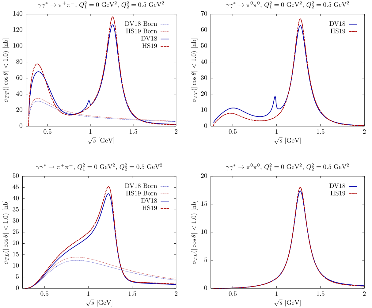
Fig. 64. Predictions for the cross section for \gamma\gamma^* \rightarrow \pi^+\pi^- (left) and \gamma\gamma^* \rightarrow \pi^0\pi^0 (right) for Q^2 = 0.5 GeV 2 from DV18 [669] and HS19 [670] compared to the Born results (dotted curves).
