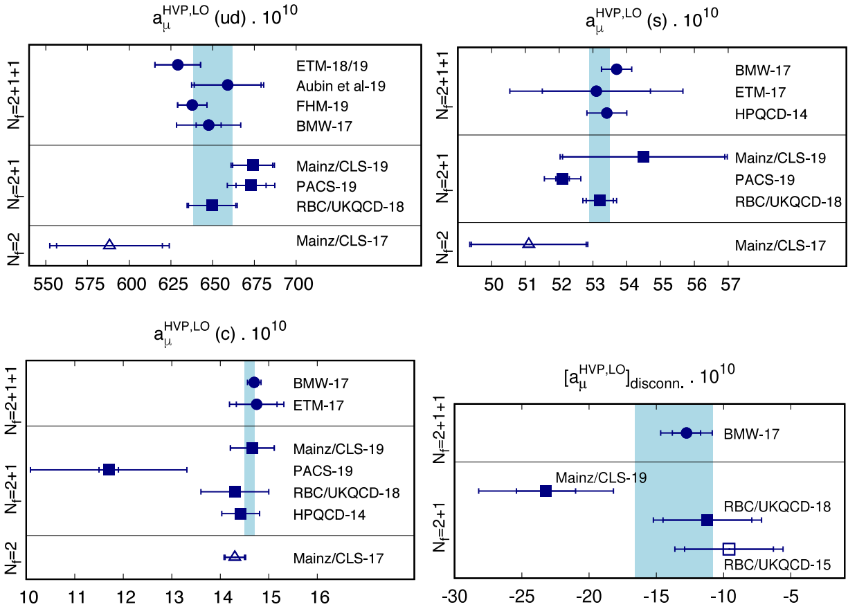
Fig. 45. Comparisons of lattice results for flavor-specific contributions to a_\mu^{\text{HVP, LO}}(\alpha^2) . (Upper-Left) Light-quark connected contribution a_\mu^{\text{HVP, LO}}(ud) . (Upper-Right) Strange-quark connected contribution a_\mu^{\text{HVP, LO}}(s) . (Lower-Left) Charm-quark connected contribution a_\mu^{\text{HVP, LO}}(c) . (Lower-Right) Quark-disconnected contribution a_\mu^{\text{HVP, LO}}|_{\text{disc.}} . The lattice results in each panel are grouped by the number of sea quarks in the gauge ensembles employed in the underlying calculations, where “ N_f = 2 + 1 + 1 ” (circles) labels ensembles with up, down, strange, and charm quarks in the sea, for “ N_f = 2 + 1 ” (squares) charm quarks are not included in the sea, while for “ N_f = 2 ”, (up triangles) strange quarks are also omitted in the sea. Filled symbols indicate results included in the lattice averages of Section 3.5.1, which are shown here as light blue bands. Open symbols indicate results that have been updated or superseded, see Table 9 for further details.
