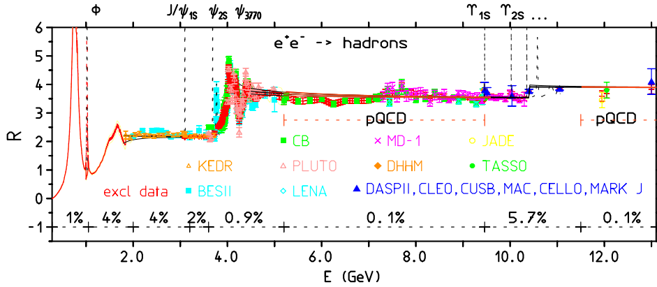
Fig. 29. The compilation of R(s) -data utilized in the analyses of Refs. [27,217–220]. The bottom line shows the relative systematic errors within the split regions. Different regions are assumed to have uncorrelated systematics. Data from Refs. [37,41,44–47,53–56,59,62,63,66,67,69–72,75–77,142,167,222–227] and others. Source: Adapted from Ref. [27].
