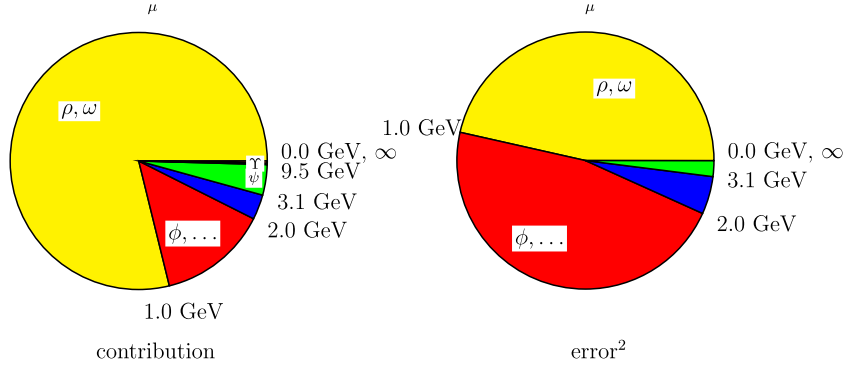
Fig. 30. Distribution of contributions and error squares from different energy regions. Source: Reprinted from Ref. [27].
