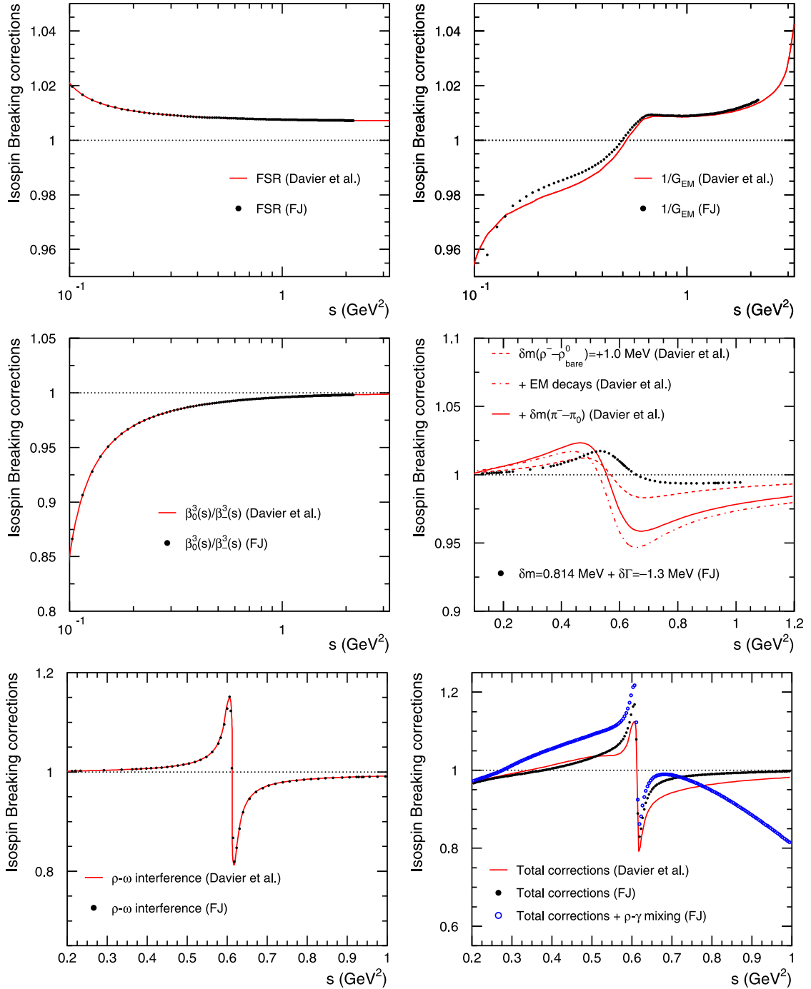
Fig. 19. Comparison of IB corrections versus s used by Davier et al. [176] and by FJ [177]. The different plots correspond to FSR (top left), 1/G_{\text{EM}} (top right), \beta_0^3/\beta_-^3 ratio term (middle left), the effect of the \rho mass and width difference in the |F_0/F_-|^2 term (middle right), the effect of the \rho - \omega interference in the |F_0/F_-|^2 term (bottom left), and the total corrections (bottom right). The difference between the open blue points and the solid black one in the last plot stems from the \rho - \gamma mixing corrections proposed in Ref. [178]. Source: Reprinted from Ref. [179].
