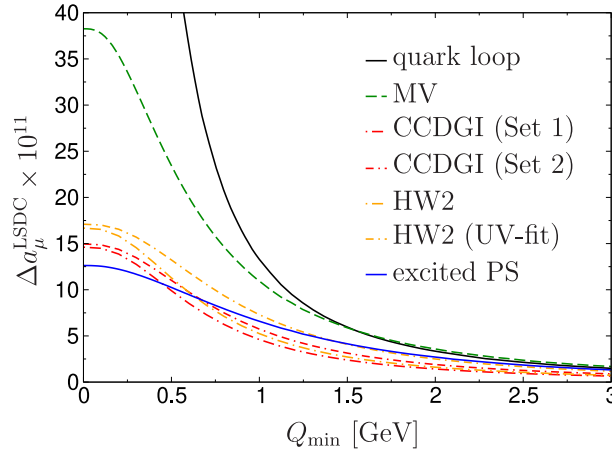
Fig. 69. \Delta a_{\mu}^{\text{LSDC}} as a function of a cut Q_{\min} \leq Q_i in the (g-2)_{\mu} integral. The quark loop diverges for Q_{\min} \rightarrow 0 (and m_q = 0 ) and is included for its asymptotic behavior, the other curves illustrate the implementations of the longitudinal SDCs discussed in the main text: MV [18,707], CCDGI [701] (two parameter sets), HW2 [700] (two variants of the HW2 model), and excited pseudoscalars [24,572].
