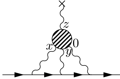
Fig. 77. Mainz definition of the coordinates x, y, z, 0 in HLbL in the (g-2)_\mu . The muon and the photon propagators are contained in the QED kernel function \tilde{\mathcal{L}} . The blob denotes the QCD correlation function i\hat{T} to be evaluated on the lattice. Source: Adapted from Ref. [720].
