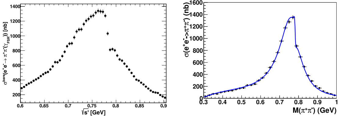
Fig. 5. The BESIII (left, reprinted from Ref. [73]) and CLEO-c (right, reprinted from Ref. [84]) data on e^+e^- \rightarrow \pi^+\pi^- in the \rho region using large-angle detected ISR photons.
