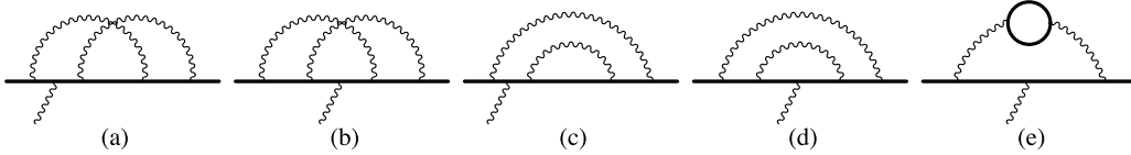
Fig. 96. Fourth-order vertex diagrams. There are seven diagrams in total. The time-reversed diagrams of (a,c) are not shown. The solid and wavy lines represent lepton and photon propagators, respectively. Source: Reprinted from Ref. [735].
