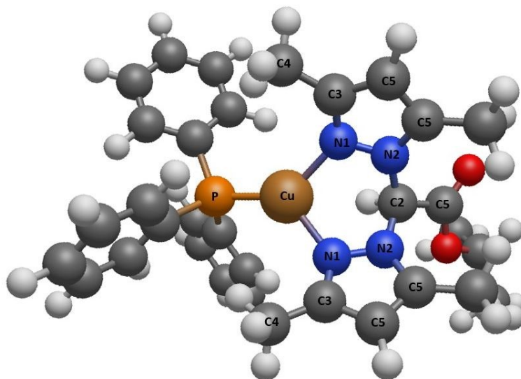
Figure 4. Optimized DFT models describing the local atomic structure around the Cu absorber for complex 3 .
