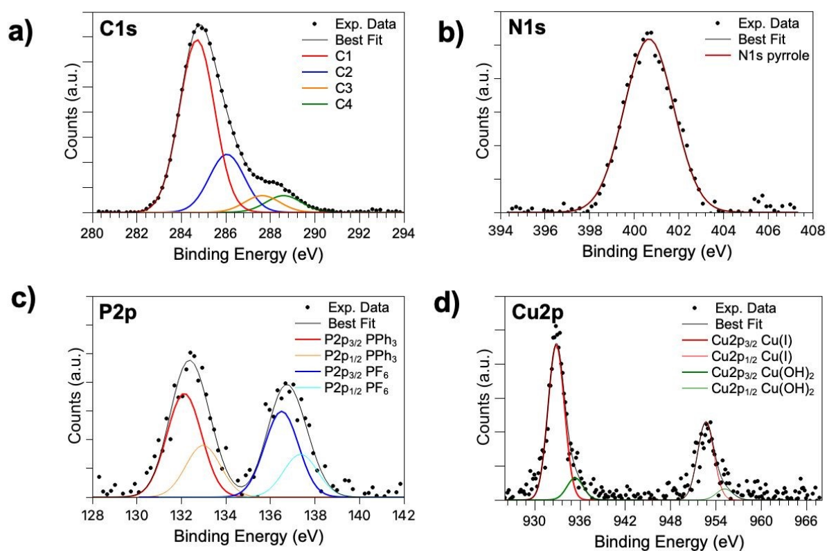
Figure 2. XPS spectra collected on complex 3 at C1s (a), N1s (b), P2p (c) and Cu2p (d) core levels.
