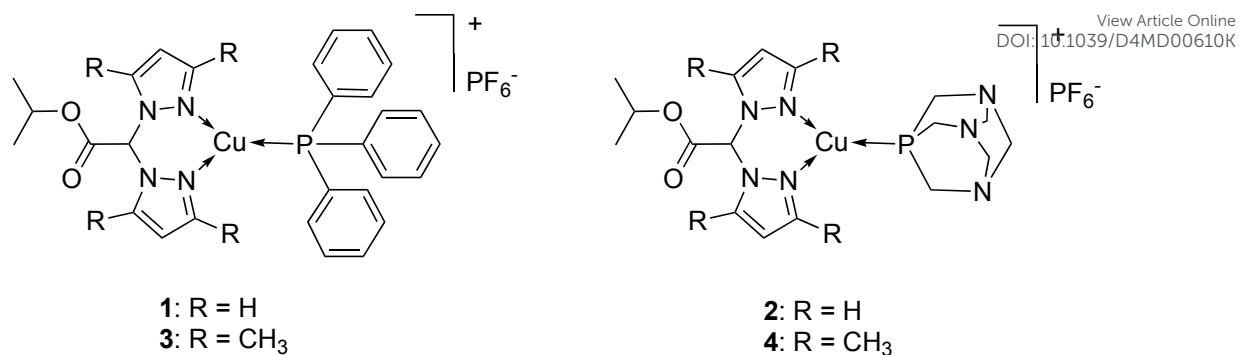
Figure 1. Chemical structures of complexes 1-4 .
