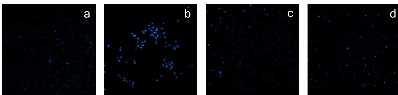
Figure 5. Hoechst staining of LoVo cells: a) control cells; b) cells incubated for 48 h with IC 50 of cisplatin; c) cells incubated for 48 h with IC 50 of 3 ; d) cells incubated for 48 h with IC 50 of 4 .
