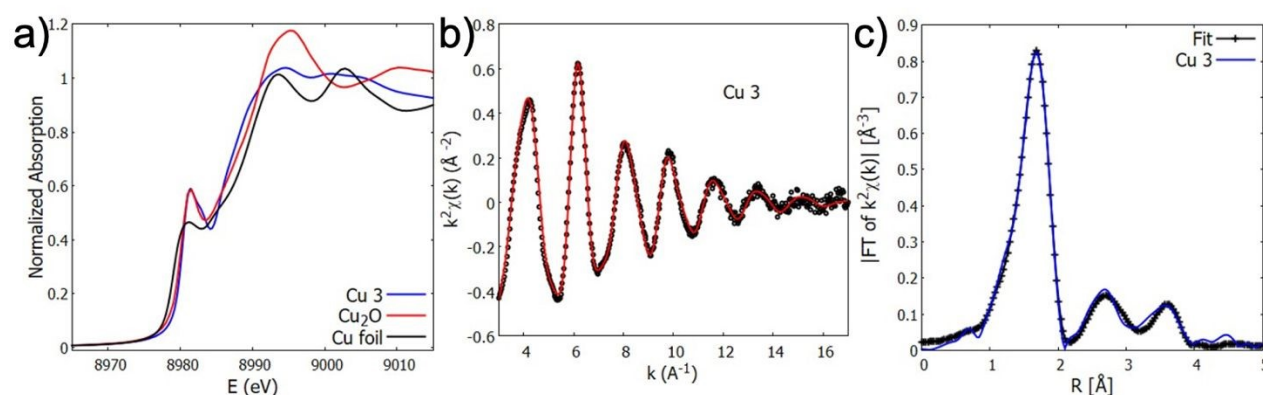
Figure 3: a) Normalized XANES spectrum of Cu K edge of 3 (blue), Cu 2 O (red) and Cu foil (black) as reference compounds. b) k 2 -Weighted experimental (black) and fit (red) curves for 3 . c) Moduli of Fourier Transforms (FT) of k 2 χ exp (k) of experimental (blue) and best fit (black) curves; the FT curves have not been corrected for the phase shift effect, resulting in a main peak shift of approximately -0.5 Å with respect to the actual distance.
