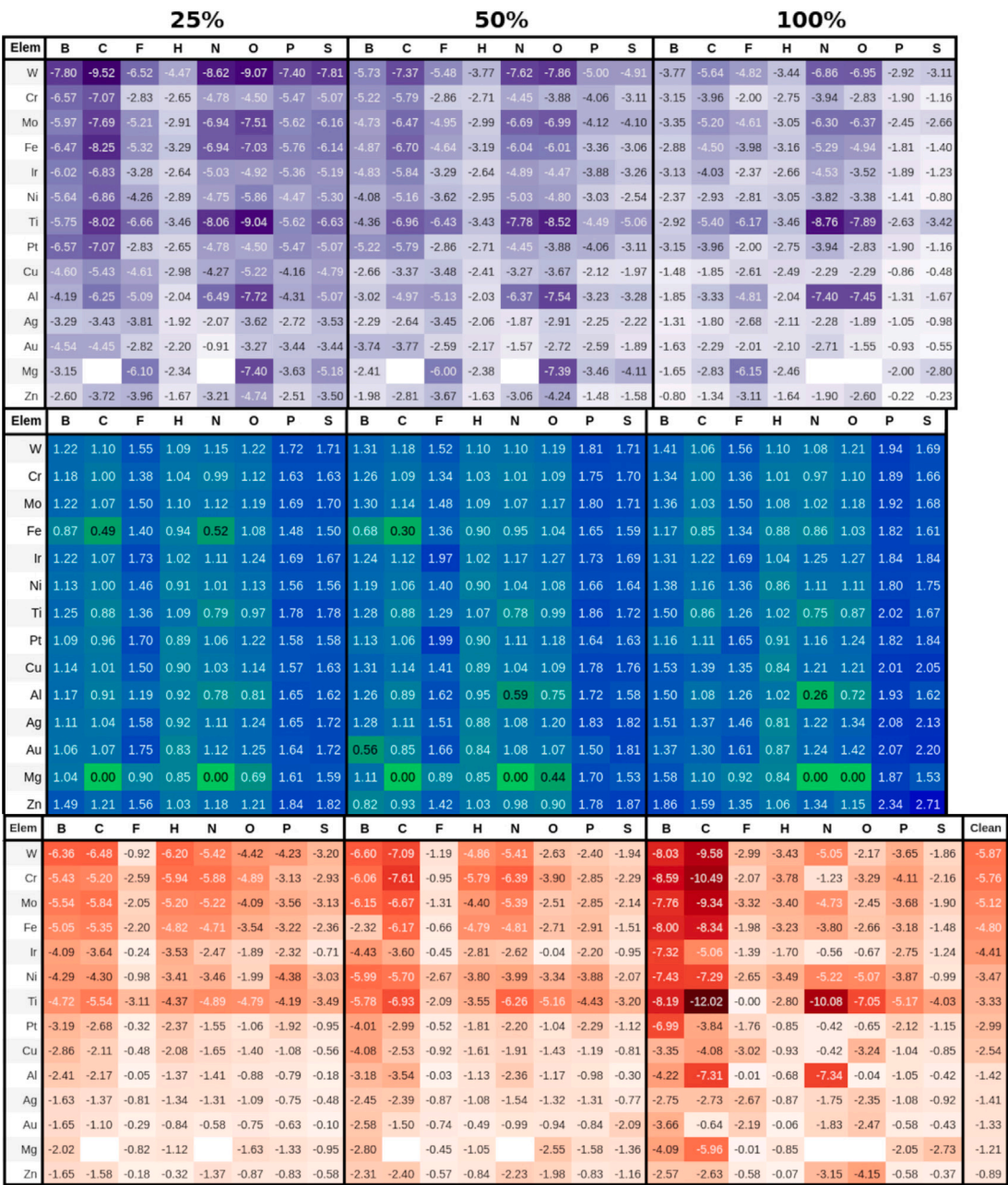
Fig. 2. Adsorption energy in eV (top panel), vertical distance along z between the adatom and the xy-plane of the substrate slab in Å (middle Panel) and adhesion energy in (J/m²) (bottom Panel) for 25%, 50% and 100% coverages. Empty squares (or with 0 value) indicates when the atomic adsorption is not stable. In this cases, the adsorbate percolates into the surface structure. For the adhesion energies the clean interfaces values calculated in Ref. [51] are reported in the Column “Clean”. In all cases darker shades are related to higher adsorption and adhesion energies.
