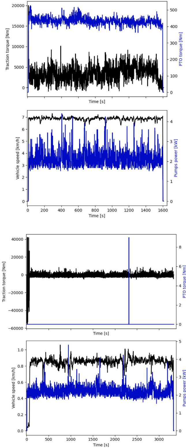
Fig. 1. Load curves: top — atomizer and bottom — tying operation.
