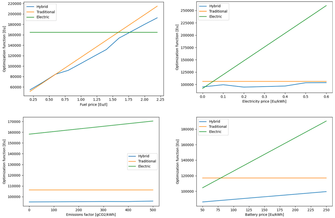
Fig. 8. Sensitivity analysis results — 1st row: fuel and electricity prices; — 2nd row: Emissions intensity factor and Battery price.
