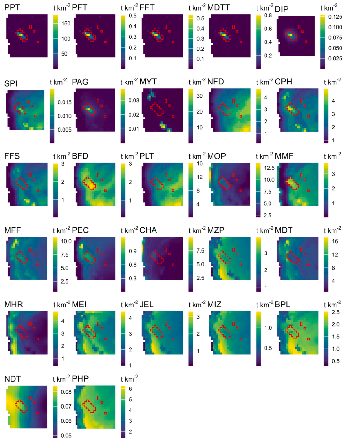
Fig. 3. Ecospace biomass outputs. Maps produced by Ecospace showing the biomass distribution ( \text{t km}^{-2} ) of the trophic groups for the baseline scenario at the steady state. In red, the borders of the SAC. Primary Producers Tegnùe (PPT), Porifers Tegnùe (PFT), Filter Feeders Tegnùe (FFT), Macrobenthic Detritivorous Tegnùe (MDTT), Diplodus annularis (DIP), Spicara smaris (SPI), Pagellus erythrinus (PAG), Mytilus galloprovincialis (MYT), Nekton Feeders (NFD), Cephalopods (CPH), Flat fish (FFS), Benthic Feeders (BFD), Planktivorous Fish (PLT), Nekton Detritivorous Feeders (NDT), Macrobenthic Predators (MOP), Macrobenthic Mixed Feeders (MMF), Macrobenthic Filter Feeders (MFF), Chamelea gallina (CHA), Pectinidae (PEC), Mesozooplankton (MZP), Macrobenthic Detritivorous (MDT), Meiobenthos (MEI), Jellyfish (JEL), Microzooplankton (MIZ), Bacterioplankton (BPL), Phytoplankton (PHP), Carcass (CAR), Detritus (DET). (For interpretation of the references to colour in this figure legend, the reader is referred to the web version of this article.)
