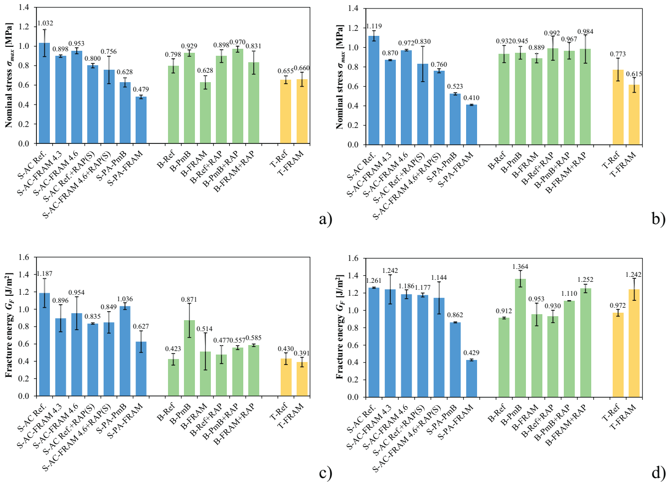
Fig. 11. SCB results and the standard deviation for a) nominal stress \sigma_{max} at -18^{\circ}\text{C} ; b) nominal stress \sigma_{max} at -24^{\circ}\text{C} ; c) fracture energy G_F at -18^{\circ}\text{C} ; d) fracture energy G_F at -24^{\circ}\text{C} ; e) fracture toughness K_{IC} at -18^{\circ}\text{C} ; f) fracture toughness K_{IC} at -24^{\circ}\text{C} ; g) Flexibility Index FI at -18^{\circ}\text{C} ; h) Flexibility Index FI at -24^{\circ}\text{C} ; i) Cracking Resistance Index CRI at -18^{\circ}\text{C} ; and j) Cracking Resistance Index CRI at -24^{\circ}\text{C} .
