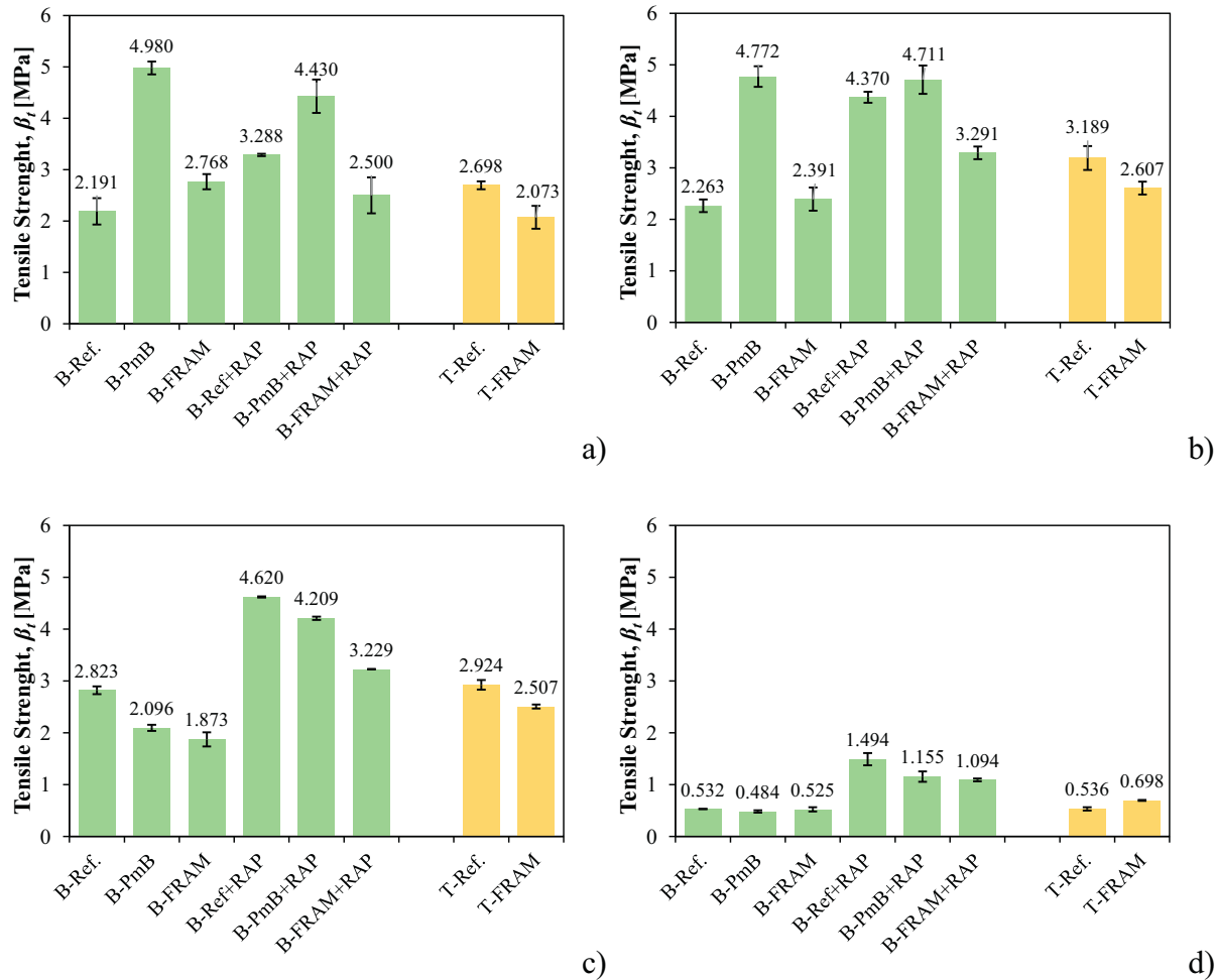
Fig. 8. UTST results and the standard deviation for a) tensile strength at -25 °C; b) tensile strength at -10 °C; c) tensile strength at 5 °C; d) tensile strength at 20 °C; e) tensile failure strain at -25 °C; e) tensile failure strain at -10 °C; g) tensile failure strain at 5 °C; and h) tensile failure strain at 20 °C.
