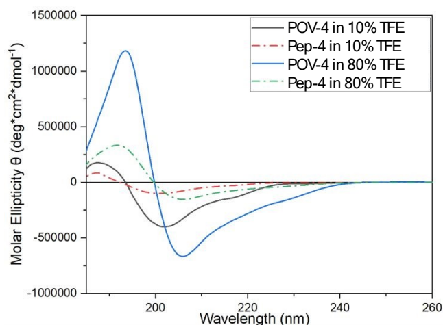
Fig. 6. Far-UV CD spectra of Pep-4 (12.5 μM, dot-dashed lines) and POV-4 (12.5 μM, solid lines) at different TFE percentage.
