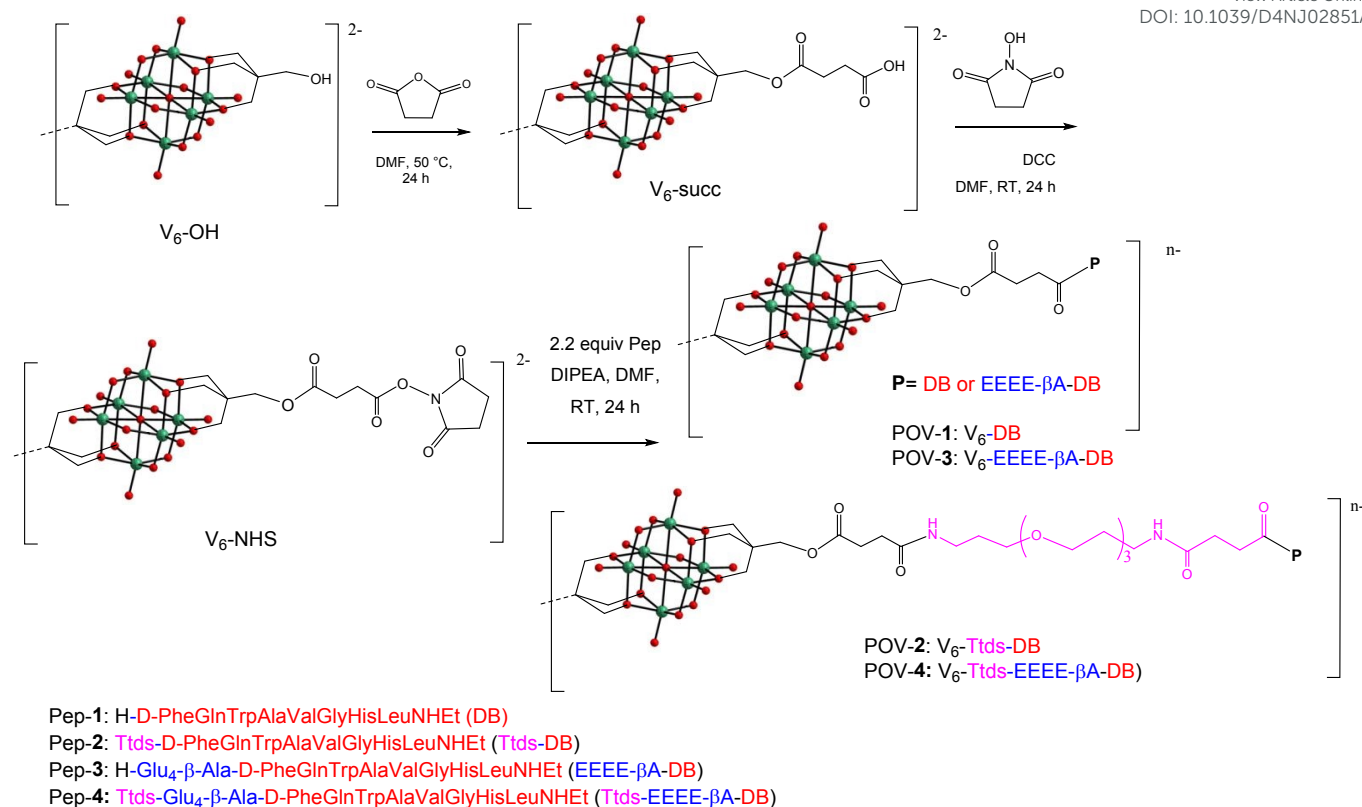
Scheme 1. Reaction scheme to obtain the hybrid derivatives starting from V 6 -OH (TBA 2 [V 6 O 13 {(OCH 2 ) 3 CH 2 OH} 2 ]). For clarity reasons, counter cations (TBA) are omitted.
