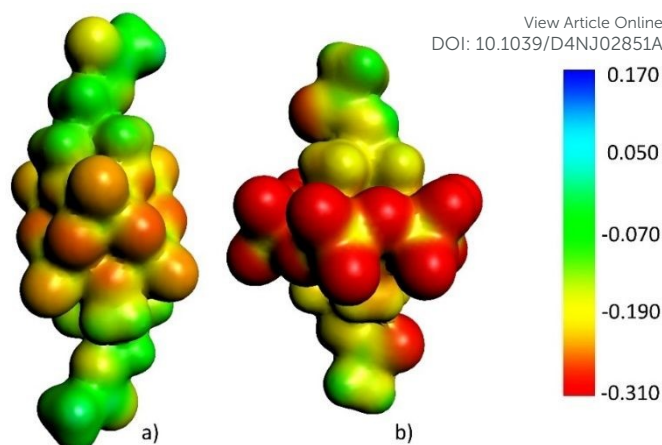
Fig. 1: DFT calculated electrostatic potential mapped on an electronic isosurface of 0.01 density for the two POM precursors: a) [V_6O_{13}\{(OCH_2)_3CNH_2\}_2]^{2-} , and b) [MnMo_6O_{18}\{(OCH_2)_3CNH_2\}_2]^{3-} . Red and blue regions indicate negative and positive potential, respectively.
