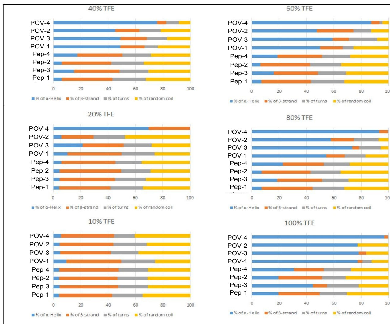
Fig. 7. Percentage of \alpha -helix (blue), \beta -strand (orange), turns (grey) and random coil (yellow) for peptides and POV-hybrids in 10%, 20%, 40%, 60%, 80% and 100 % TFE solution.
