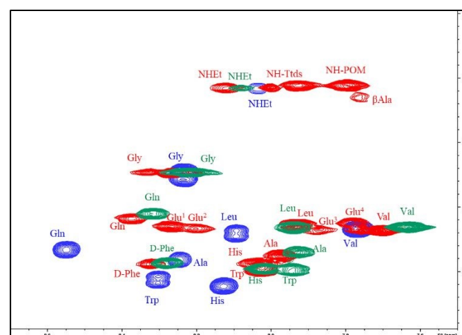
Fig. 4: Overlaid COSY spectra (in \text{d}_6\text{-DMSO} ) for NH- \text{CH}\alpha cross peaks belonging to free and \text{V}_6 -grafted DB (Pep-1 (blue), POV-1 (green) and POV-4 (red)). The spectra were acquired on a Bruker DMX-600 instrument operating at 599.90 MHz for ^1\text{H} at 298 K.
