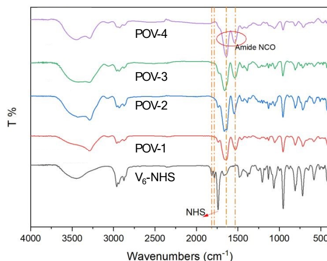
Fig. 2. FTIR (KBr) spectra of V 6 -NHS (black), POV-1 (red), POV-2 (blue), POV-3 (green), POV-4 (purple), the orange dash-dot lines indicate the position of the characteristic peaks at 1814 cm -1 , 1783 cm -1 , 1640 cm -1 and 1534 cm -1 (see text).
