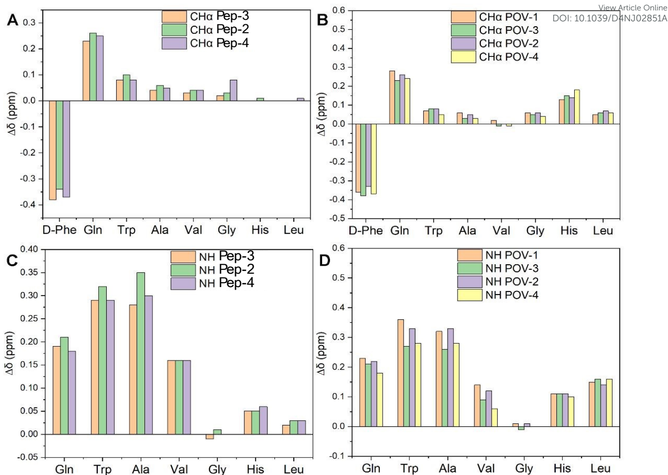
Fig. 5. Influence of the POV-spacers on chemical shift of peptide. \Delta\delta values were determined by subtracting the resonances of DB-spacer or POV-spacer-DB hybrids to the resonances of DB. A) and C) are \Delta\delta of DB-spacers, B) and D) are \Delta\delta of POV-spacers-DB.
